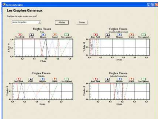
Figure 8: The L-R fuzzy numbers used in the software.
