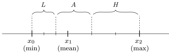
Figure 6: Splitting the intervals.
