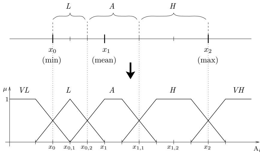
Figure 7: Building the fuzzy classes.
