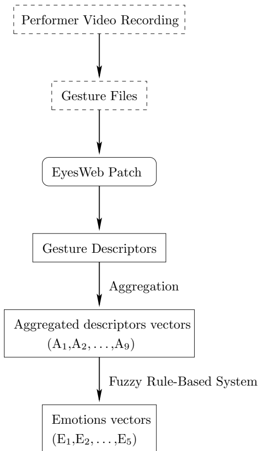
Figure 4: Our system components.
