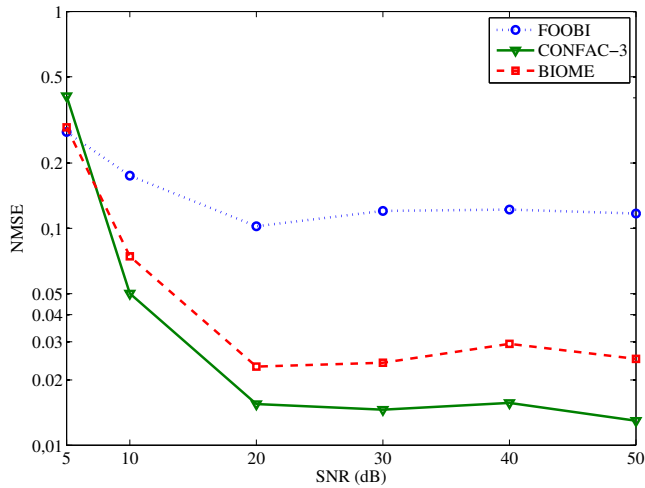
Fig. 1. NMSE vs. SNR ( K = 5 , N = 3 , M = 5000 , S = 100 )
