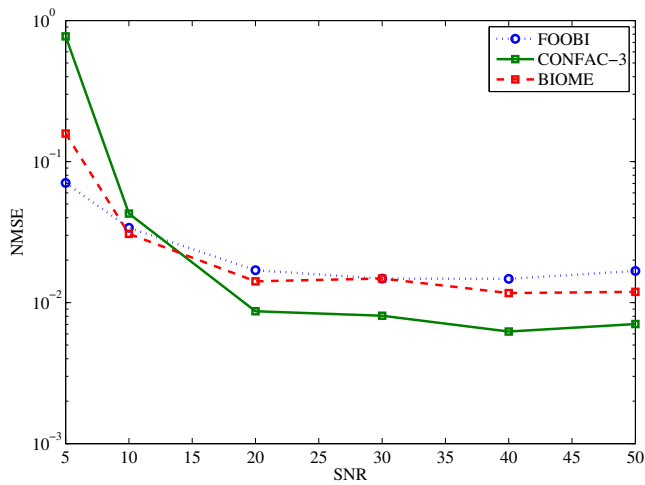
Fig. 2. NMSE vs. SNR ( K = 7 , N = 4 , M = 20000 , S = 100 )
