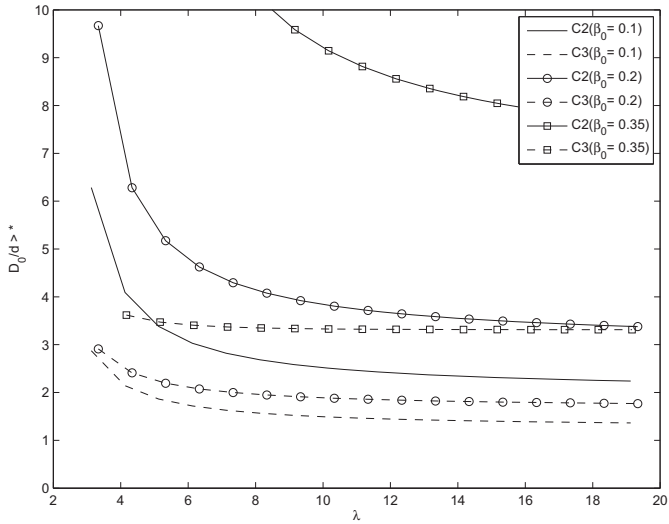
Fig. 2. Thresholds for conditions C2 and C3 to hold, for \beta_0 = 0.1, 0.2, 0.35 .
