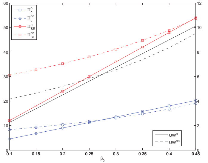
Fig. 3. \Pi_c , \Pi_{SE} and UW for neutral and non-neutral cases ( D_0/d = 6, \lambda = 8 )
