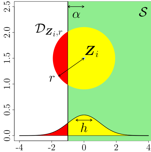
FIGURE 5. Link between \mathbb{P}(\mathbf{Z}_i + \boldsymbol{\varepsilon} \in \mathcal{S}) and \mathcal{A}(\mathcal{D}_{\mathbf{Z}_i, r} \cap \mathcal{S}) where \mathcal{S} is a half-plane.
