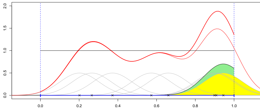
FIGURE 2. Weight correction of a density on [0, 1] : kernel K is no longer a Gaussian density, but a truncated Gaussian density.
