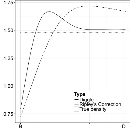
(a) \mathbb{E}(\hat{f}), n = 100
