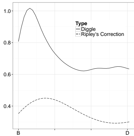
(c) \sqrt{\text{Var}(\hat{f}), n = 100}
