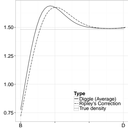
(b) \mathbb{E}(\hat{f}), n = 1000
