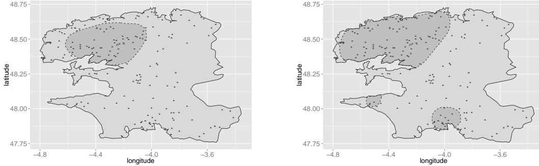
FIGURE 12. Convex hull of hot spot areas, without border correction (on the left) and with Ripley's correction (on the right).
