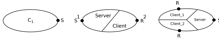
Fig. 2. Left: CC style with a single interface S. Middle: CC with two roles, cardinality, and location. Right: CC com with two roles and three hosts.
