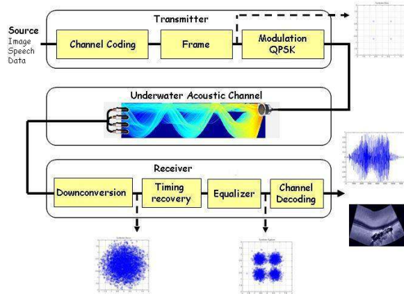
Figure 1: All-digital receiver
