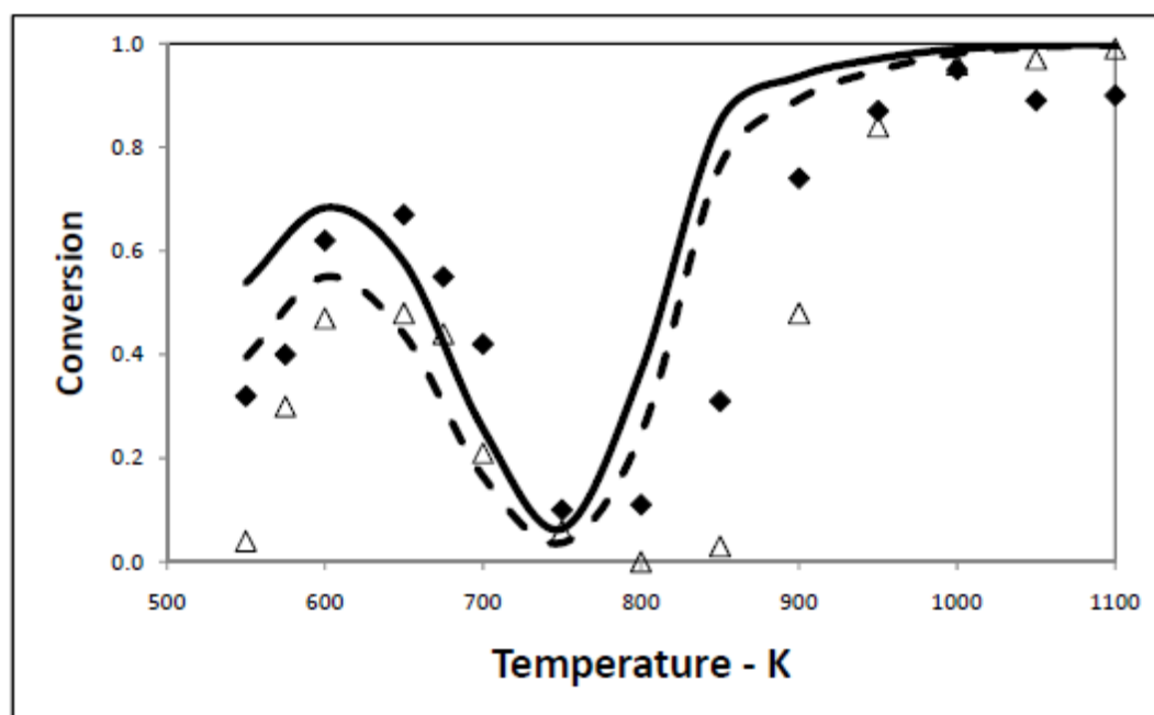
Fig. 2. Fractional conversion of methyl palmitate and n-decane in a JSR. Lines are computed results for methyl palmitate (solid line) and n-decane (dashed line), symbols show measured values from Hakka et al. [47] for methyl palmitate (diamonds) and n-decane (triangles). Mixture has 0.002 total mole fraction fuel (0.26 methyl palmitate/0.74 n-decane), stoichiometric with O_2 , diluted by helium, atmospheric pressure.
