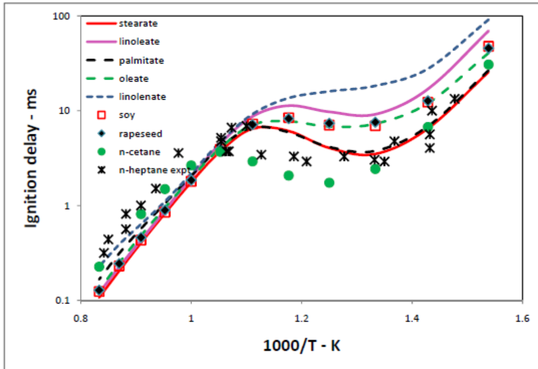
Fig. 10. Ignition delay times for stoichiometric fuel/air mixtures in a reflected shock environment, 13.5 bar initial pressure. Experimental results [66] for n-heptane/air are shown by asterisks, other results are kinetic model predictions. Lines show predicted values for each methyl ester fuel, circles for n-cetane [41], squares and diamonds are predictions for SME and RME.
