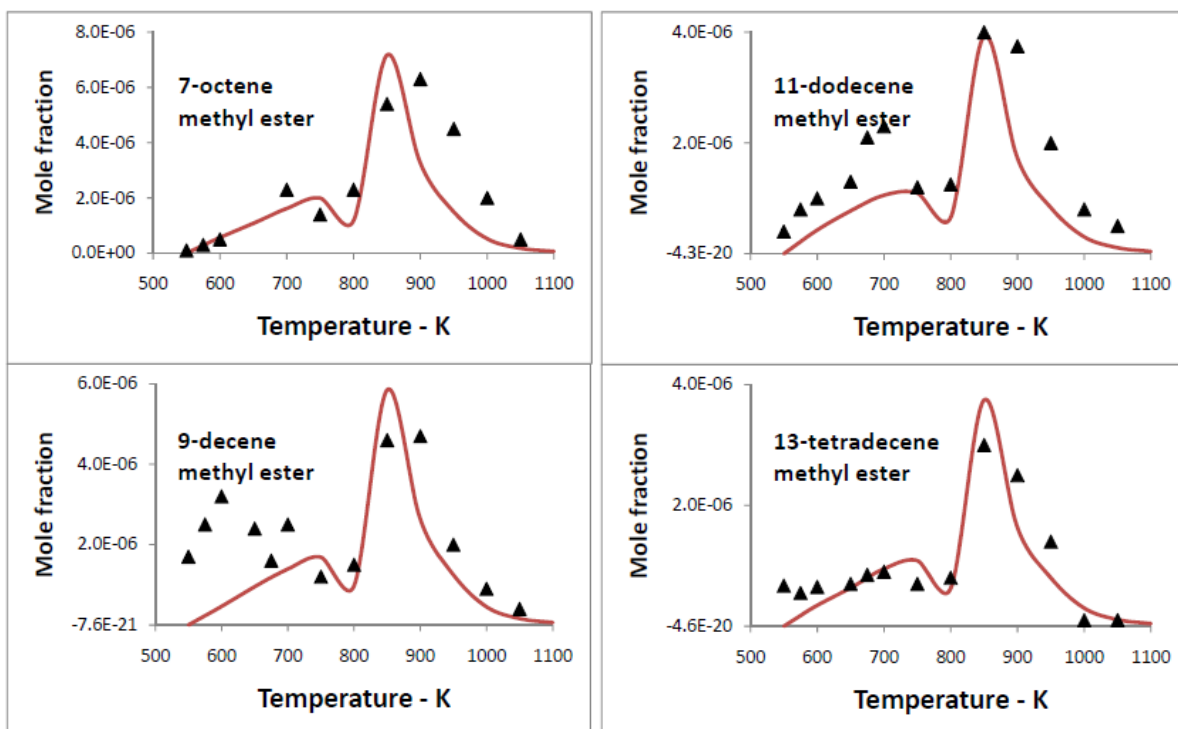
Fig. 4. Comparisons between experimental results from Hakka et al. [47] (symbols) and computed values (lines) for selected 1-olefin methyl ester species with the conditions shown in Fig. 2.
