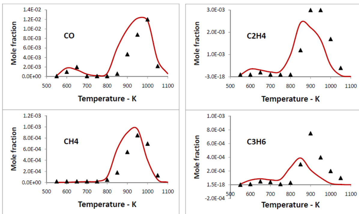
Fig. 6. Comparisons between experimental results from Bax et al. [48] (symbols) and computed values (lines) for selected major intermediate species with the conditions shown in Fig. 5.
