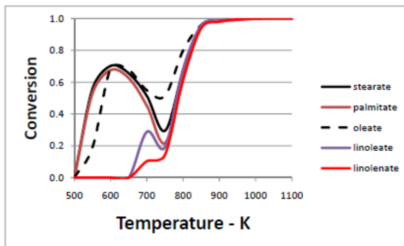
Fig. 8. Computed fuel fractional conversions for five separate simulations, each with a different methyl ester fuel. The fuel in each case is given in the legend, for stoichiometric fuel/oxygen, 0.2% fuel, with helium diluent, residence time 1.5 s.
