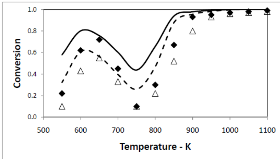
Fig. 5. Fractional conversion of methyl oleate and n-decane in a JSR. Lines are computed results for methyl oleate (solid line) and n-decane (dashed line), symbols show measured values from Bax et al. [48] for methyl oleate (diamonds) and n-decane (triangles). Mixture has 0.002 total mole fraction fuel (0.26 methyl oleate/0.74 n-decane), stoichiometric with O_2 , diluted by helium, atmospheric pressure.
