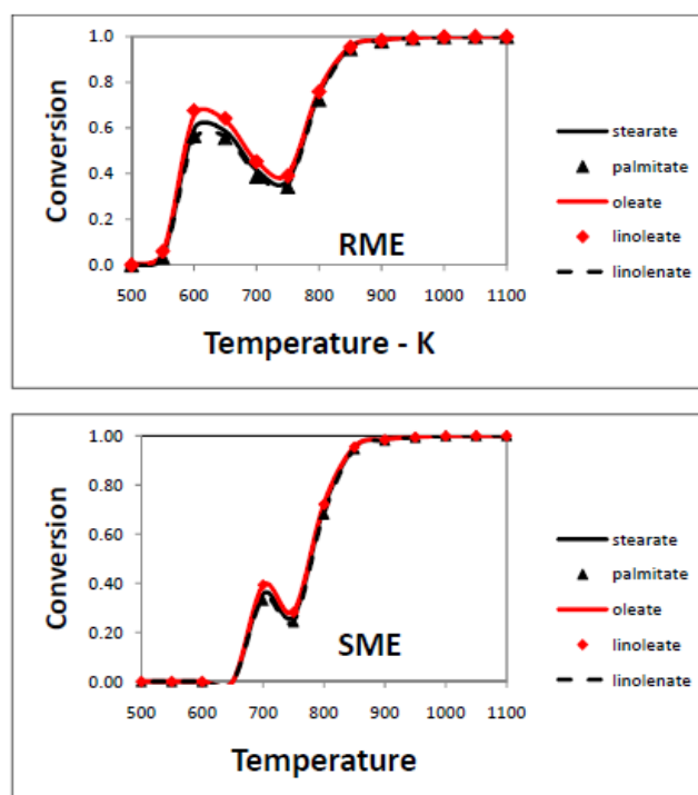
Fig. 9. Computed comparison between oxidation of RME and SME in a simulated JSR, stoichiometric fuel/oxygen, 0.2% fuel, diluted in helium, residence time 1.5 s. The RME and SME compositions taken from Table 1.
