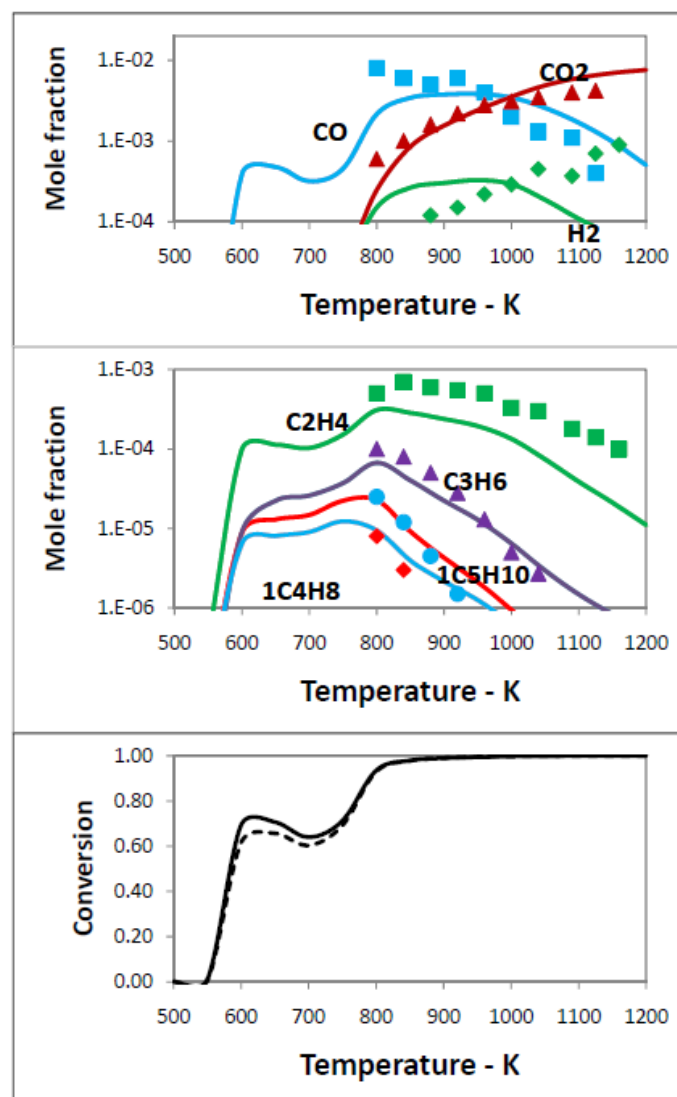
Fig. 7. Comparisons between experimental results (symbols) from Dagaut et al. [34] and computed results for RME oxidation in JSR at 10 bar pressure, stoichiometric RME/O 2 with 0.05% fuel, diluted in N 2 and with a residence time of 1 s. Also shown are computed fractional fuel conversions for methyl oleate (solid curve) and methyl palmitate (dashed curve).
