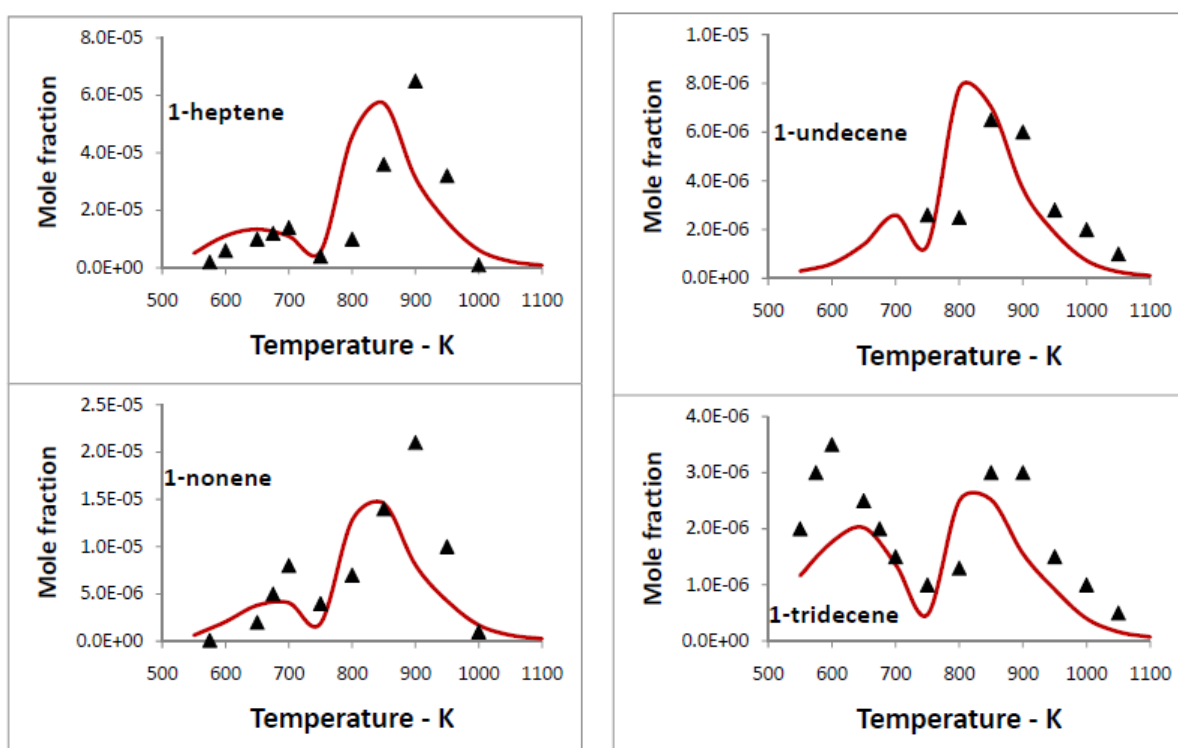
Fig. 3. Comparisons between experimental results from Hakka et al. [47] (symbols) and computed values (lines) for selected 1-olefin species with the conditions shown in Fig. 2.
