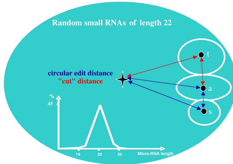
Fig. 12 The set of the random small RNAs of length equal to the mean (22) of the lengths of 319 human micro-RNAs (histogram bottom), with indication of the barycenters of the t RNA loops set (t), ancestral RNA rings set A (a) and real small RNAs set (s)
