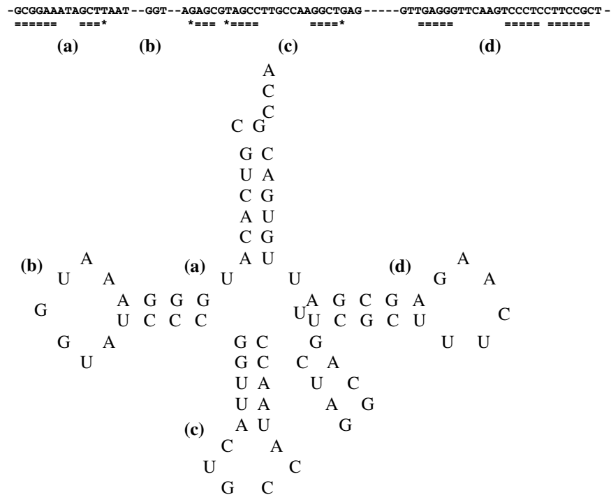
Fig. 6 Primary sequence of Gly- 1 RNA of Oenothera lamarckiana (top) and RNA ring of length 72 in cloverleaf secondary structure (bottom)
