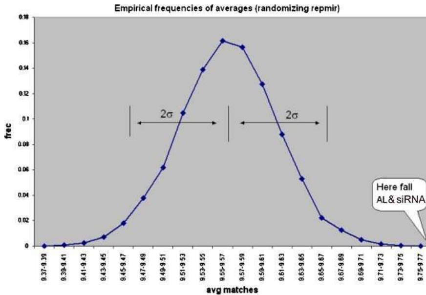
Fig. 11 Histogram of match averages between micro-RNAs repeated in at least 2 different species (repmirs) and random small RNAs of length 22 having the same base frequencies than AL. The average matches between the repmirs and AL, and between HDV siRNA targets and AL are indicated at the right part of the curve
