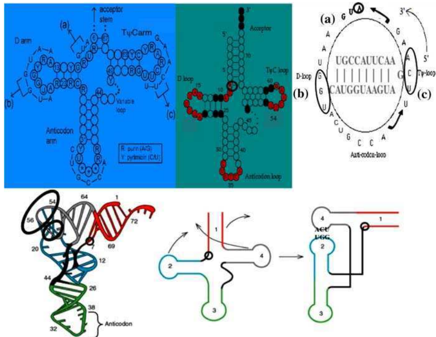
Fig. 5 Plausible primitive 3 RNA AL in ring and hairpin secondary structures (top right); 3 RNA with invariant loops coming from Gly- 3 RNA of Arabidopsis thaliana (top centre); correspondence with AL (top left); 3 RNA ternary structure (bottom left) with base 7 (A) as pivot (bottom centre) in an identical position as on AL between the dual ACU and UGG triplets responsible for the loops 2 and 4 association (bottom right)
