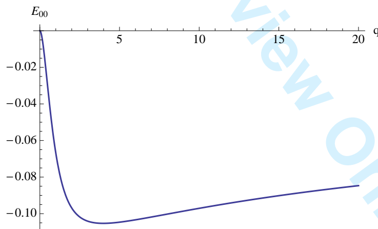
Figure 2. The ground state energy of the total Hamiltonian, Eq. (19), versus q . The minimum occurs at q_{\min} = 3.918 and E_{00}(q_{\min}) = -0.105 , cf. Table 1.
