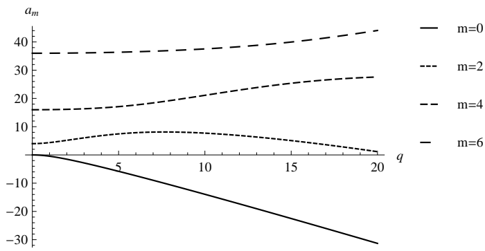
Figure C2. The eigenvalues of a_m(q) of the Mathieu function ce_m versus q .
