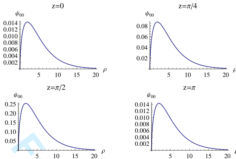
Figure 3. The ground state eigenfunction \psi_{00}(\rho, z, q_{\min}) with q_{\min} = 3.918 , cf. Eq. (16) and Table 1.
