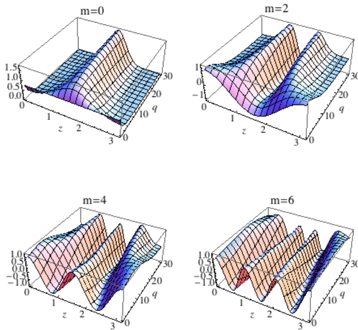
Figure C1. The Mathieu function ce_m(a_m, q, z) for several even values of m over the plane (z, q) .
