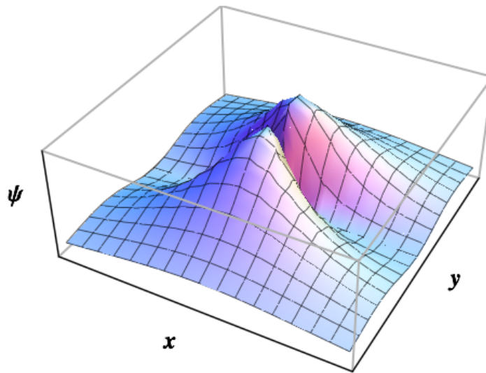
Figure 4. The distribution of the ground state eigenfunction \psi \equiv \psi_{00}(\rho, \vartheta, q_{\min}) with q_{\min} = 3.918 , cf. Eq. (16) and Table 1, corresponding to the spatial variation of order parameter near the edge dislocation. Here x = \rho \cos \vartheta and y = \rho \sin \vartheta .
