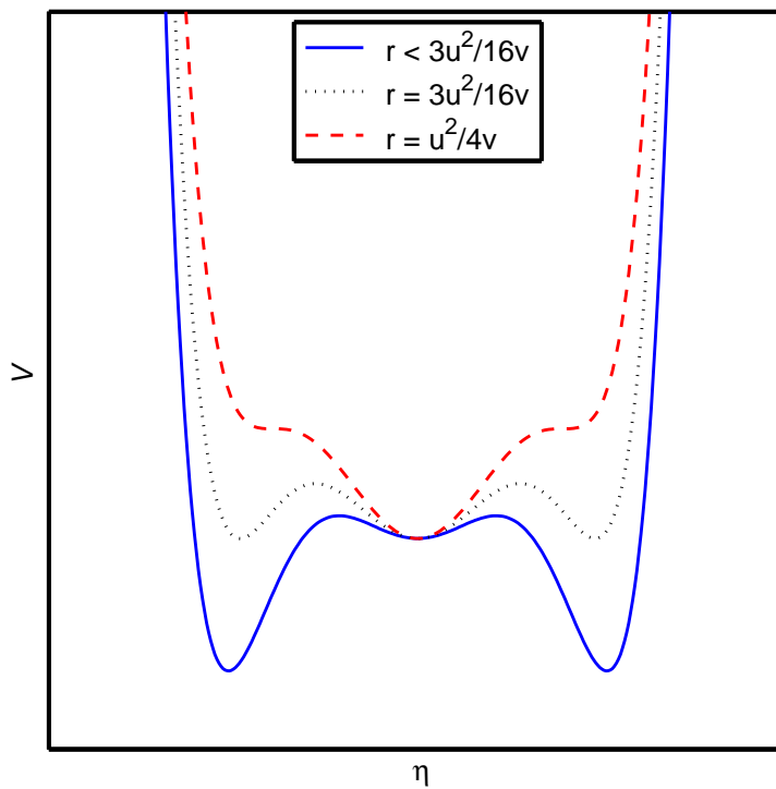
Figure 6. The Landau potential energy \mathcal{V} = \frac{r}{2}\eta^2 + \frac{u}{4}\eta^4 + \frac{v}{6}\eta^6 , with v > 0 , u < 0 , r > 0 , and \eta scalar. The curves determine the lines plotted in figure 5. The dashed curve marks the emergence of metastable second-phase II (two local minima) in the parent phase I (global minimum); the dotted line indicates that phases I and II are equally stable; and the solid line infers to when phase I is less stable than phase II, which remains in that state until r \leq 0 .
