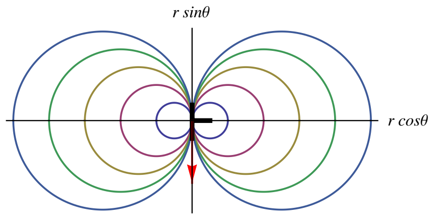
Figure 1. Equipotentials of an edge dislocation with interaction energy given by Eq. (1). The downward arrow indicates the Burgers vector.
