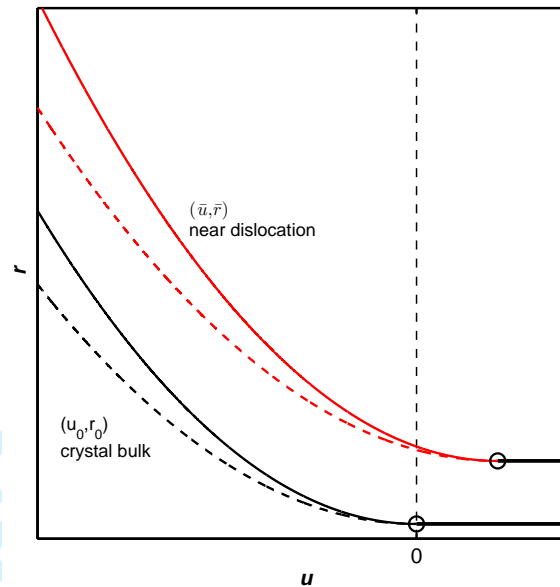
Figure 5. Phase diagram of nucleation in the bulk of rigid crystal (u_0, r_0) and near the edge dislocation (\bar{u}, \bar{r}) obtained from Landau's potential (see figure 6). The dashed line describes the first order transition, the solid line the border of instability, and the open circles are the tricritical points.
