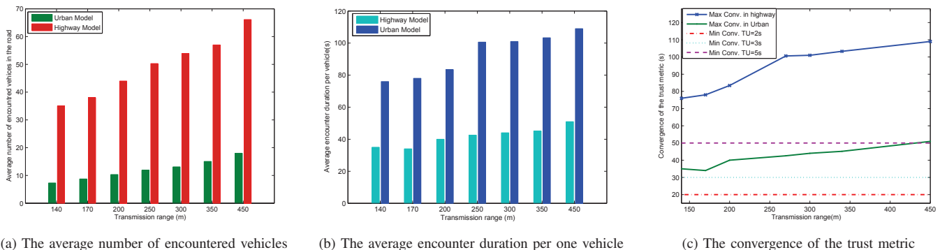
Fig. 5. The average number of encountered vehicles, the average encounter duration and the convergence of the T_m in highway and urban models
