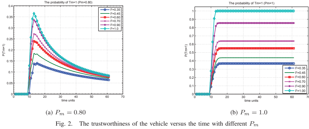
Fig. 2. The trustworthiness of the vehicle versus the time with different P_m
