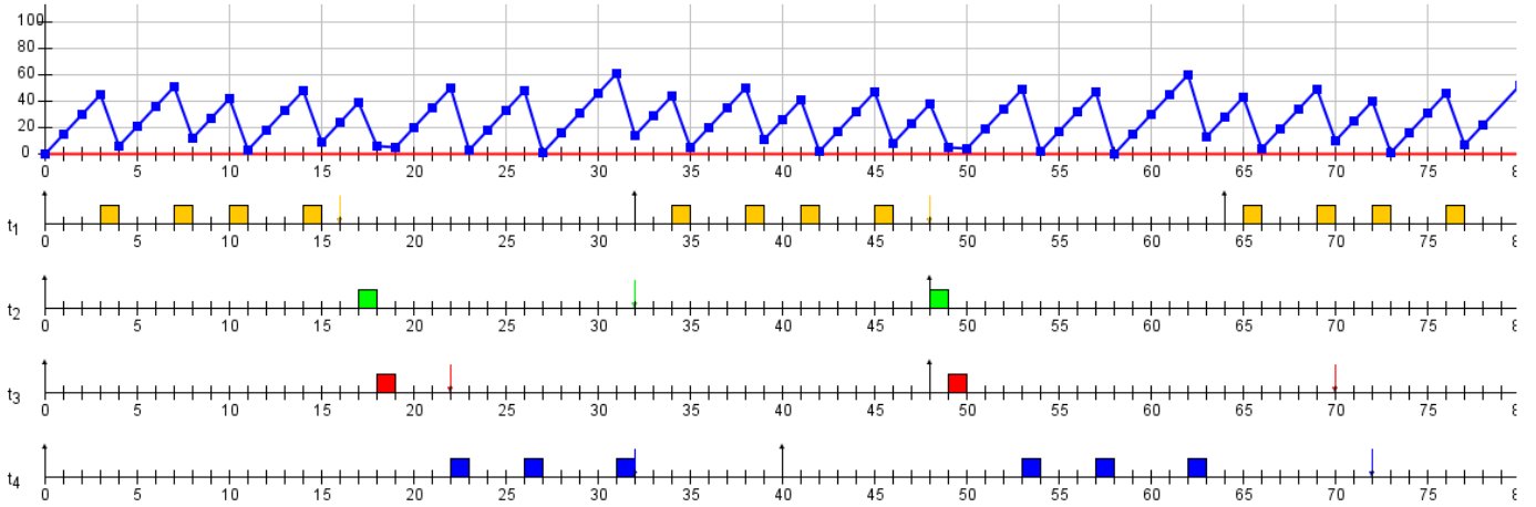
Figure 3. PFPP_{ALAP} is not optimal
