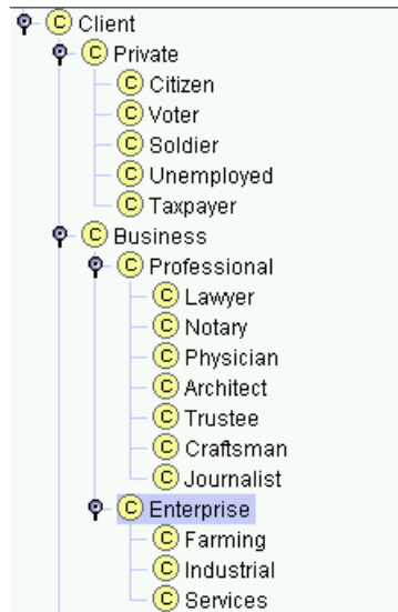
Figure 11: Class hierarchy
