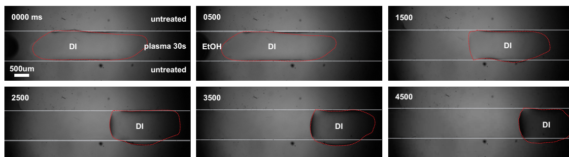
Fig. 2. Picture sequence showing from above the actuation of the water droplet by an ethanol droplet on an hydrophilic highway.
