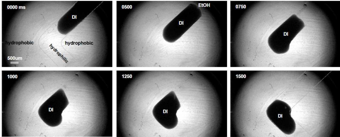
Fig. 5. Distilled water droplet forced around a 90^\circ corner.
