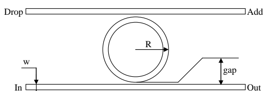
Figure 1: Microring resonator filter shape.
