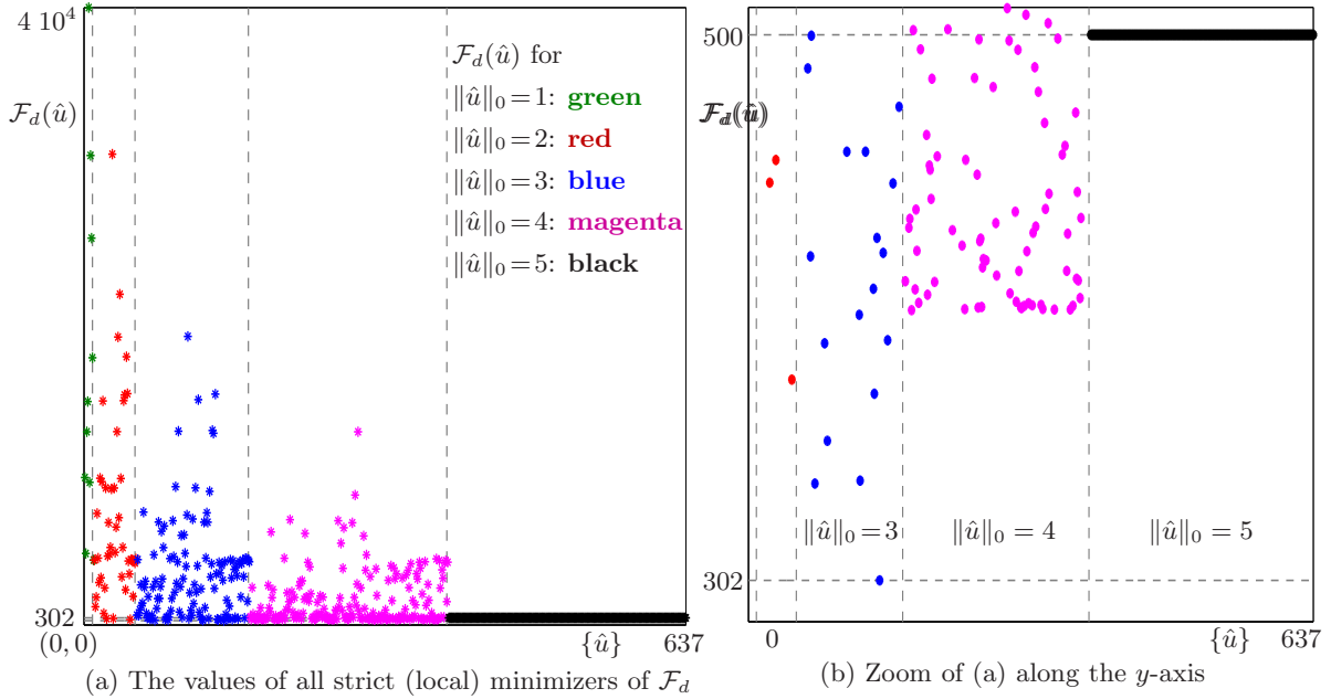
Figure 2: All 638 strict (local) minima of \mathcal{F}_d in (52) for \beta = 100 and data d corrupted with the arbitrary noise in (54). The x -axis lists all strict (local) minimizers \{\hat{u}\} of \mathcal{F}_d sorted according to their \ell_0 -norm \|\hat{u}\|_0 in increasing order. (a) The y -axis shows the value \mathcal{F}_d(\hat{u}) of these minimizers marked with a star. The value of \mathcal{F}_d for \hat{u} = 0 is not shown because it is too large ( \mathcal{F}_d(0) = 60559 = \|d\|^2 ). (b) A zoom of (a) along the y -axis. It clearly shows that \mathcal{F}_d has a very recognizable unique global minimizer
