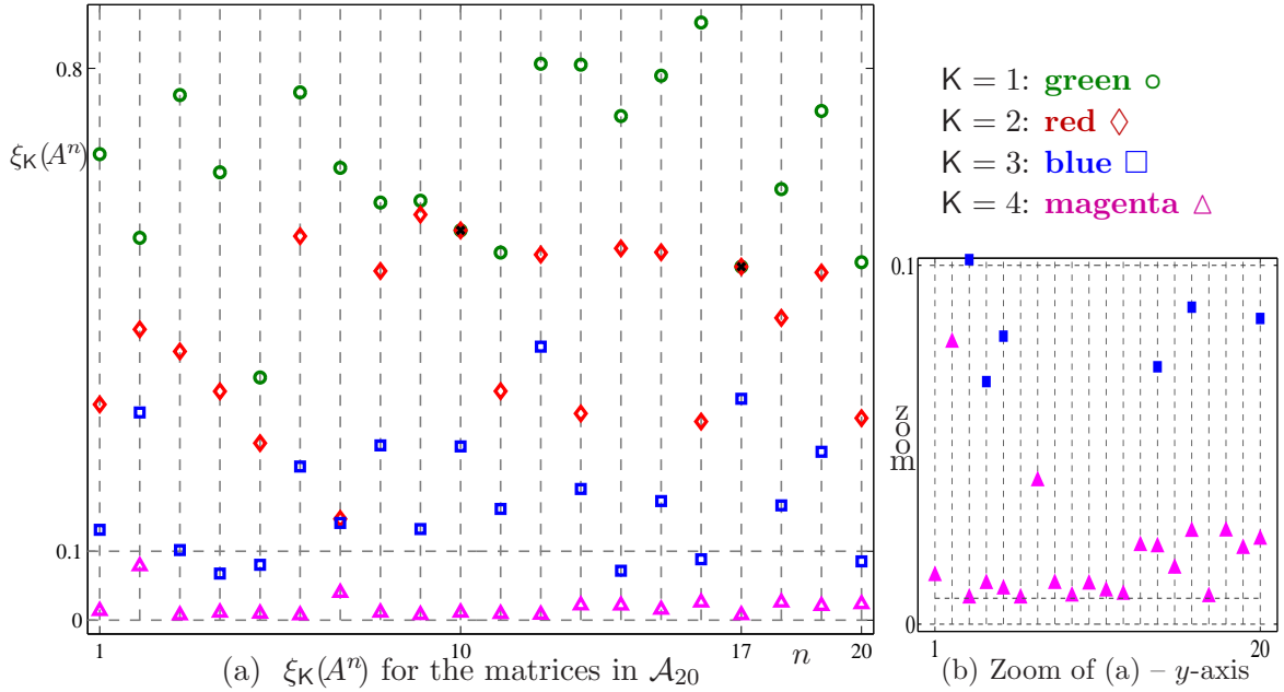
Figure 1: x -axis: the list of the 20 random matrices in \mathcal{A}_{20}^N . (a) y -axis: the value \xi_K(A^n) according to (49) for all K \in \mathbb{I}_{M-1} and for all n \in \mathbb{I}_{20} . The plot in (b) is a zoom of (a) along the y -axis.
