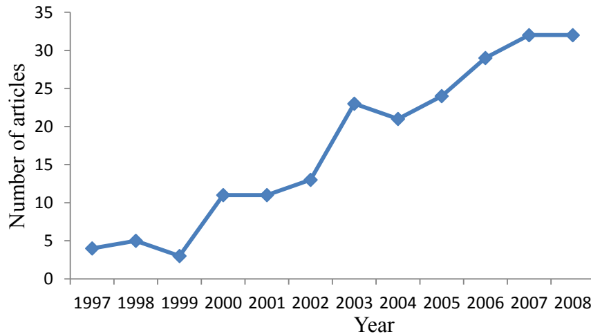
Figure 2 Publication trend
