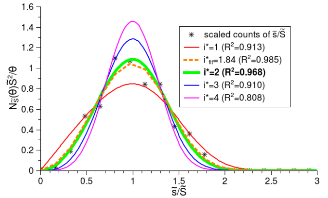
Fig. 7. Island-size histogram from the sample grown at 373 K. About 430 islands were analyzed by the model of ISD [10] and supplemented with the ISD for several values of i^* for comparison. The dashed line is a least square fit to the data of the histogram. The thick line marks the selected i^* .
