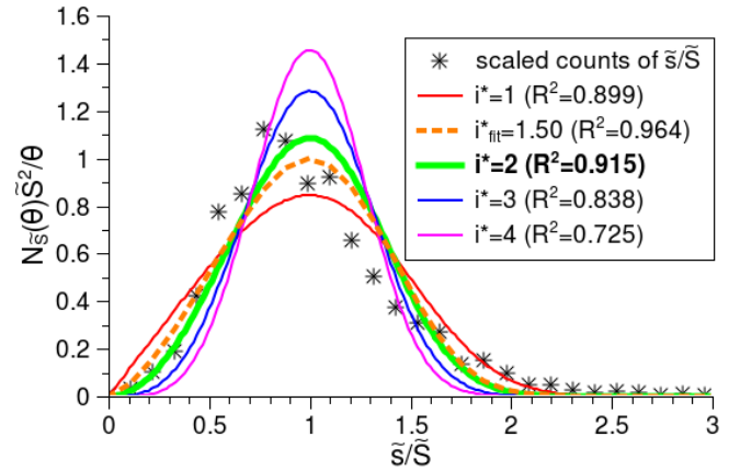
Fig. 4. Island-size histogram obtained from the sample grown at RT. The same data set of about 2700 islands was analyzed by the model of Amar-Family [10] and overlaid by fits for several i^* . The dashed line is a least square fit to the data of the histogram. The thick line marks the selected i^* .
