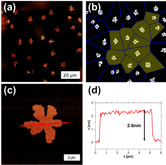
Fig. 5. a) 85 \times 85 \mu\text{m}^2 AFM image of a sample grown at 373 K with a z-scale of 5 nm. b) Image masked with the calculated Voronoi polygons (yellow areas mark the used ones). (c) 10 \times 10 \mu\text{m}^2 AFM image of a single island. (d) Corresponding height profile represented by the red line in (c).
