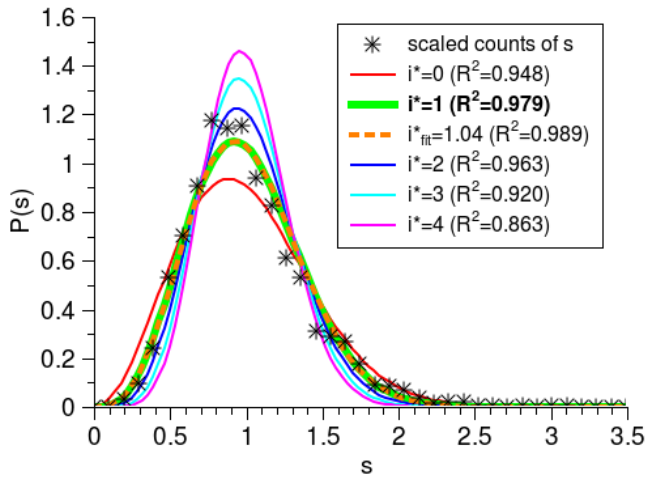
Fig. 3. Capture-zone histogram obtained from the sample grown at RT. About 2700 capture-zone areas were analyzed. Capture-zone distribution for several values of i^* are plotted for comparison. The dashed line is a least square fit to the data of the histogram. The thick line marks the selected i^* .
