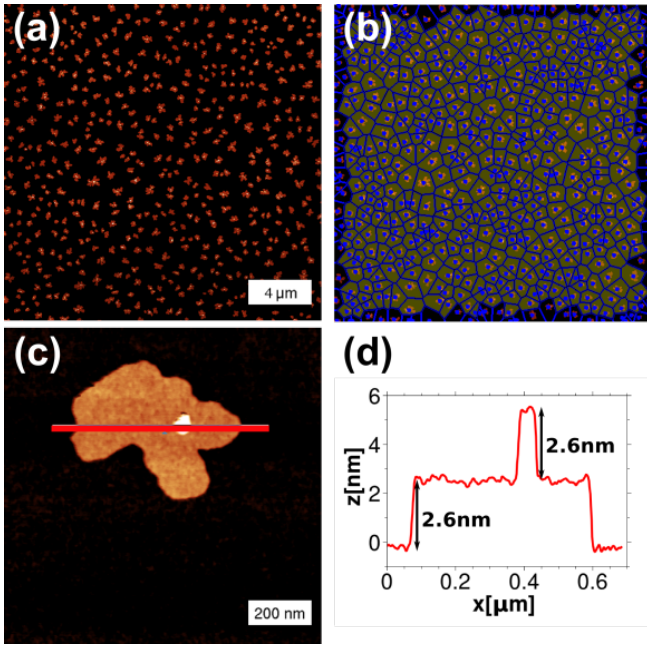
Fig. 2. (a) 20 \times 20 \mu\text{m}^2 AFM image of a sample grown at RT with a z -scale of 5 nm. (b) Image masked with the calculated Voronoi polygons. (c) 1 \times 1 \mu\text{m}^2 AFM image of a single island. (d) Corresponding height profile represented by the red line in (c).
