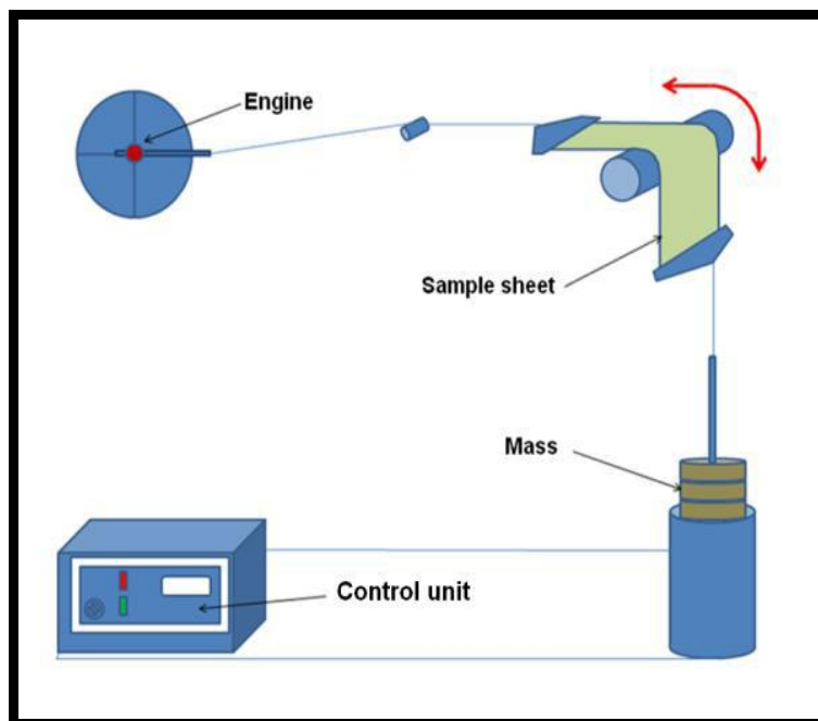
Fig.5: bending fatigue machine. Different curvature radii can be used (5 mm, 10 mm and 25 mm) with a maximum speed of 15 cycles by min.
