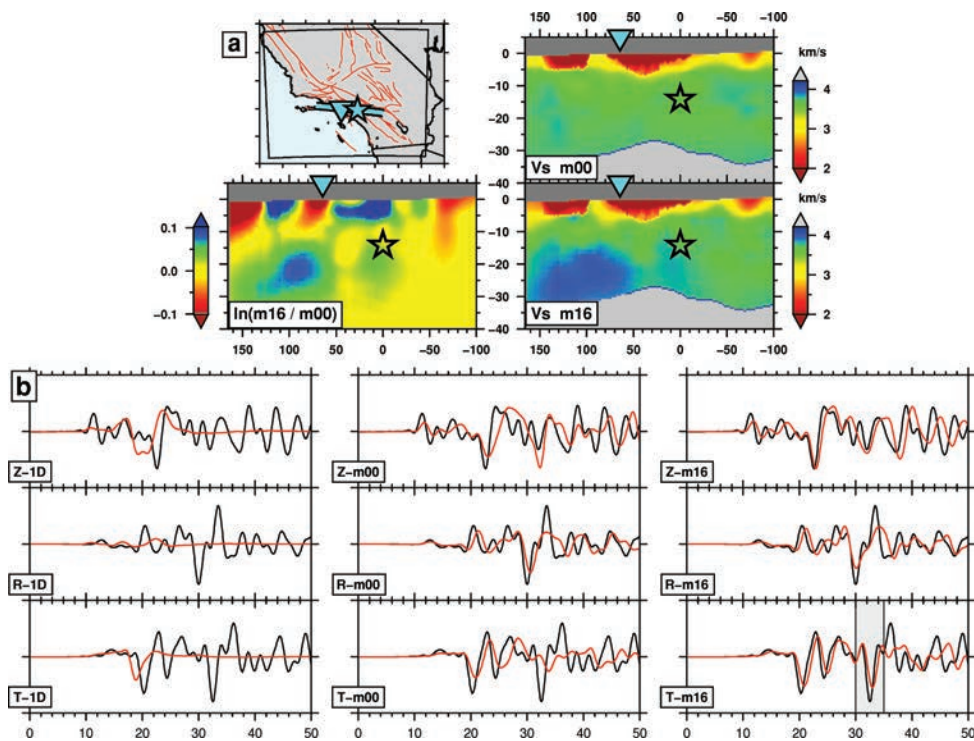
Figure 15. Vertical cross-sections and corresponding three-component seismograms (Section 5.2.1). (a) Cross-section of the V_S tomographic models for a path from event 14383980 (*; M_w 5.4, depth 14.2 km), beneath the Chino Hills region of Los Angeles, to station SMS.CI (∇; distance 64.6 km), near the northwest margin of the Los Angeles basin. (b) Synthetic seismograms (red) and observed seismograms (black) for the period range 2–30 s. The grey window on the transverse component highlights a seismic waveform discussed in Section 5.2.1. See Fig. 9 caption for explanations of subplots. This earthquake was not used in the tomographic inversion.
