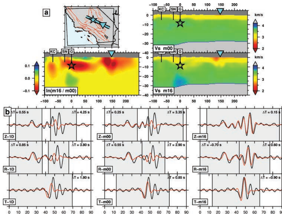
Figure 9. Vertical cross-sections and corresponding three-component seismograms (Section 5.2.1). (a) Cross-section of the V_S tomographic models for a path from event 14418600 ( \star ; M_w 3.9, depth 8.5 km), on the Garlock fault, to station HEC.CI ( \nabla ; distance 147.3 km), in the eastern Mojave Desert. Upper right panel is the initial 3-D model, \mathbf{m}_{00} , lower right panel is the final 3-D model, \mathbf{m}_{16} , and lower left panel is the difference between the two, \ln(\mathbf{m}_{16}/\mathbf{m}_{00}) . KC, Kern Canyon fault; SN, Sierra Nevada fault; G, Garlock fault. (b) Synthetic seismograms (red) and observed seismograms (black) for the period range 6–30 s. The left column shows synthetics computed using a 1-D model for southern California. The centre column shows synthetics computed using our initial 3-D model \mathbf{m}_{00} . The right column shows synthetics computed using our final 3-D model \mathbf{m}_{16} . Z, vertical component, R, radial component, T, transverse component. In this example, the highlighted time windows, each with a corresponding \Delta T travelt ime difference, are automatically selected for measurement using the FLEXWIN algorithm (Maggi et al. 2009). This earthquake was not used in the tomographic inversion.
