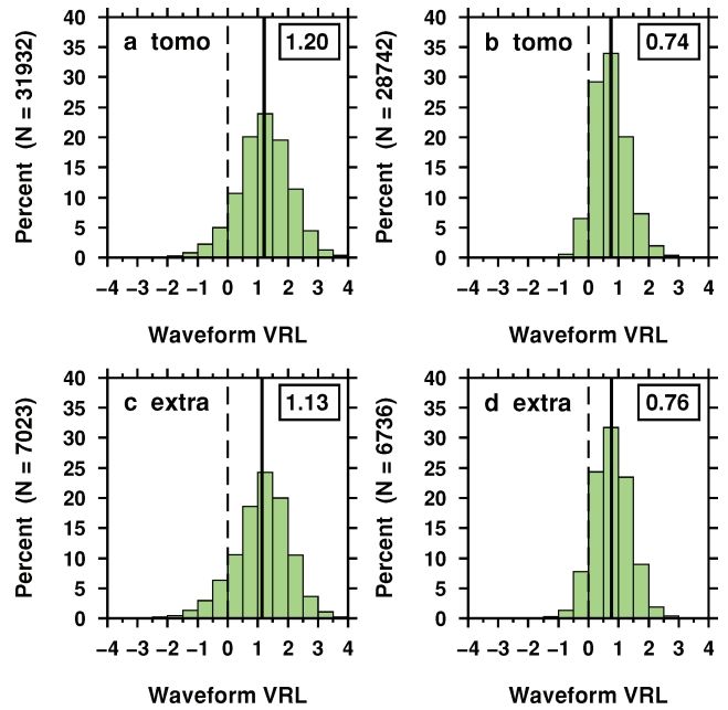
Figure 22. Same as Fig. 21, but showing logarithmic variance reduction, VRL, instead of variance reduction, VR. The quantities are approximately Gaussian distributions with the mean value denoted by the vertical black line and indicated by the boxed number. The range of permissible values of VRL is from -\infty to \infty . A value of VRL = 0 corresponds to no reduction in misfit.
