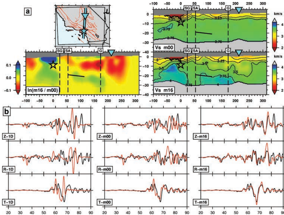
Figure 16. Vertical cross-sections and corresponding three-component seismicograms (Section 5.2.1). (a) Cross-section of the V_S tomographic models for a path from event 9818433 ( \star ; M_w 4.4, depth 8.6 km), east of the Los Angeles basin, to station CLC.CI ( \nabla ; distance 211.7 km), north of the Garlock fault. Vertical lines denote surface positions of faults: San Gabriel (SG), San Andreas (SA), and Garlock (G). Also shown for reference is a northward dipping layer identified in the wide-angle refraction survey of Fuis et al. (2001). Counter interval is 0.25 \text{ km s}^{-1} . (b) Synthetic seismicograms (red) and observed seismicograms (black) for the period range 2–30 s. See Fig. 9 caption for explanations of subplots.
