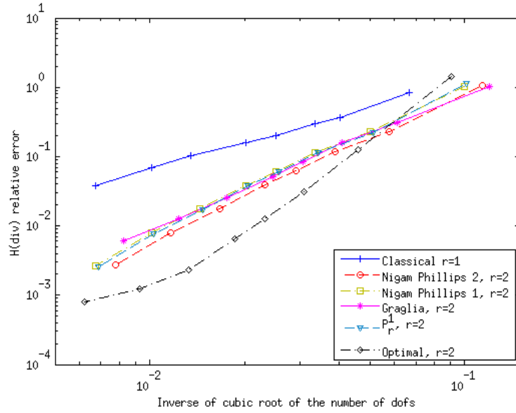
Figure 4: Relative H(\text{div}) error for different pyramidal spaces for the source problem with affine pyramids.
