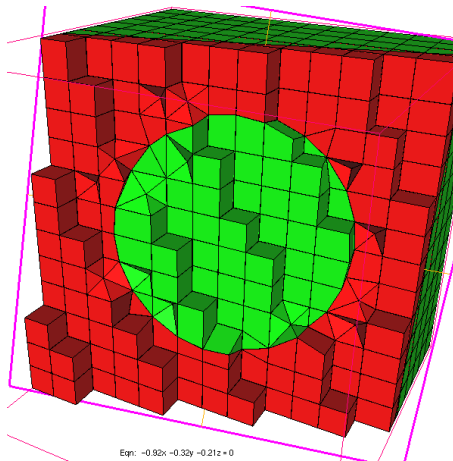
Figure 14: Hybrid mesh used for the sphere
