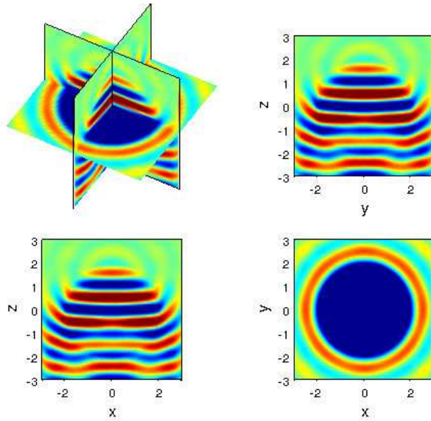
Figure 13: Divergence of u of diffracted field (real part) for the sphere.
