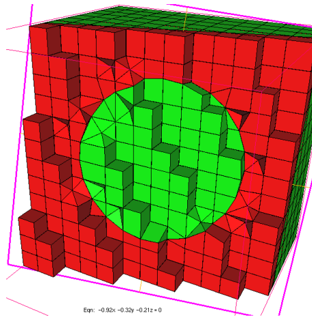
Figure 14: Hybrid mesh used for the sphere
