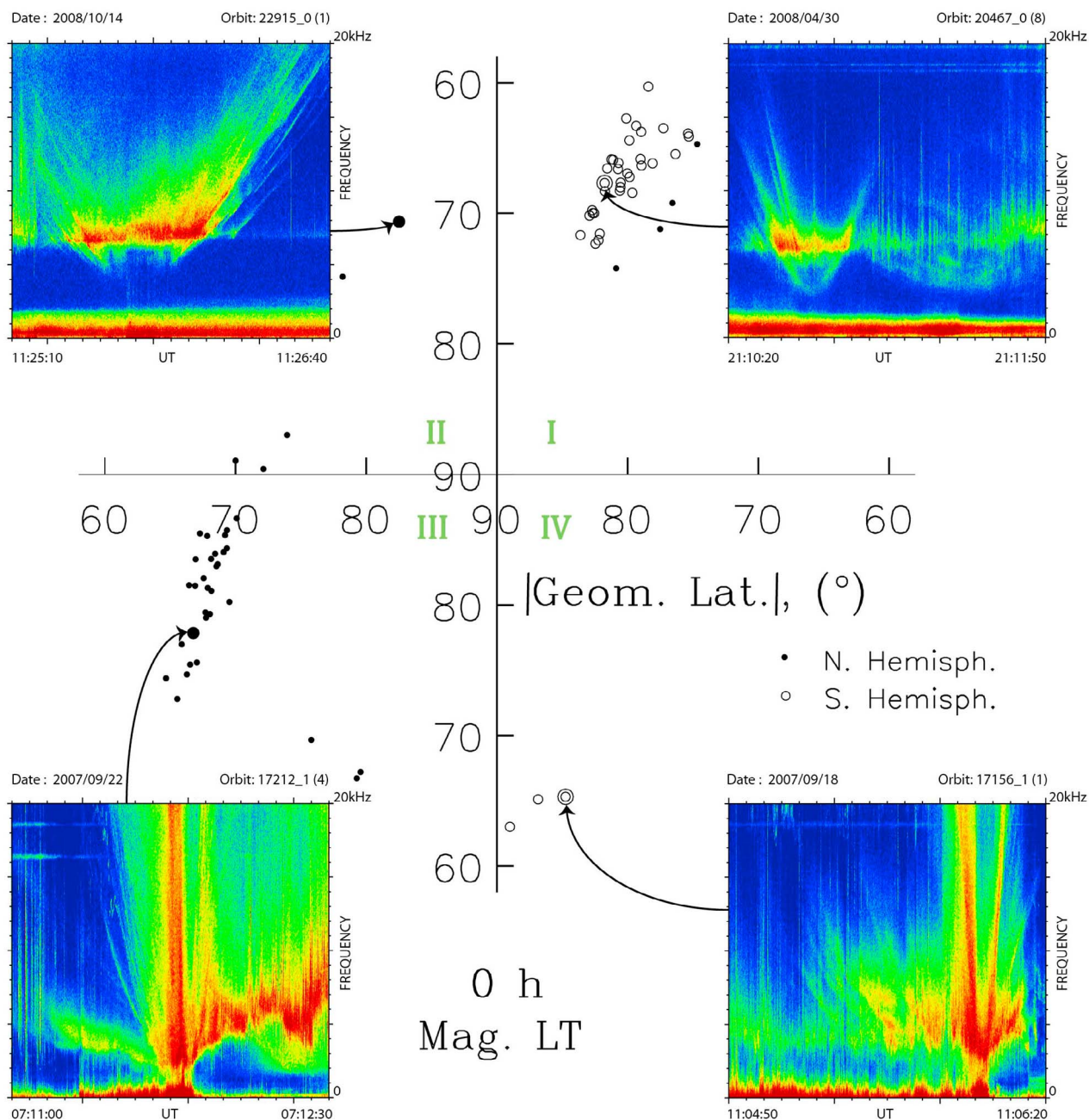
Figure 1. Distribution of saucer locations in magnetic local time and geomagnetic latitude, with spectrograms of typical saucers. Magnetic local time increases azimuthally in counterclockwise sense from 0 h at the bottom. The magnitude of the geomagnetic latitude decreases radially from 90° at the center of the plot.
