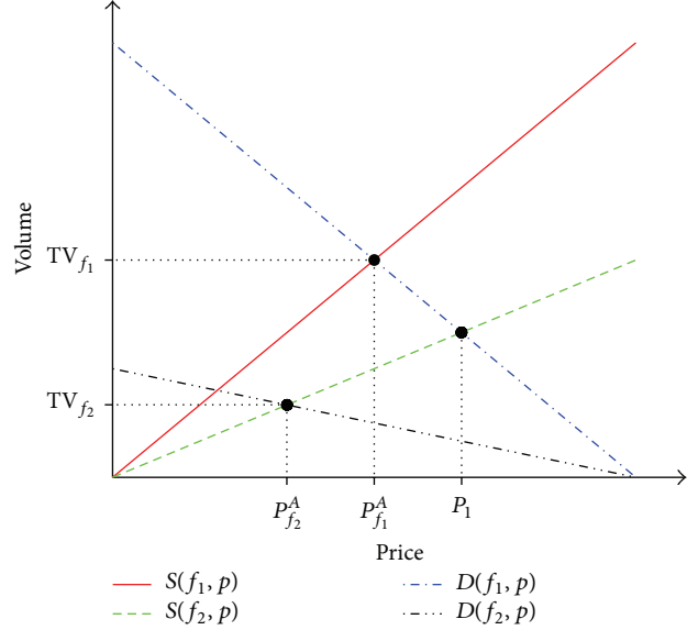
FIGURE 2: Illustration of the proof of Theorem 20.
