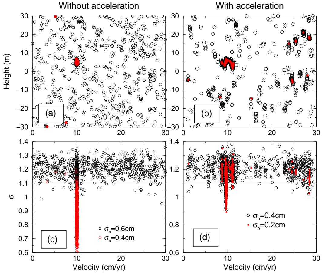
Fig. 4. (a) (b): Distribution of retrieved DEM error and velocity that maximize coherence without and with acceleration ( 0.5\text{ cm/yr}^2 ). (c) (d): Residual phase standard deviation as a function of the retrieved velocity without and with acceleration. Different colours represent different Gaussian noise levels added to the synthetic phase series. Each point corresponds to one of the 1000 random tests.
