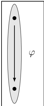
f' = \varphi \circ f is the composition of a flow and a small perturbation, r = 4
