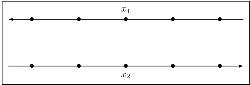
f is the time one map of the Reeb flow, r = 2
