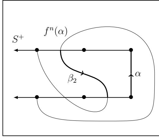
Hypothesis of proposition 3.2: -\underline{\alpha} \in \text{cut} \underline{f^n \alpha}
