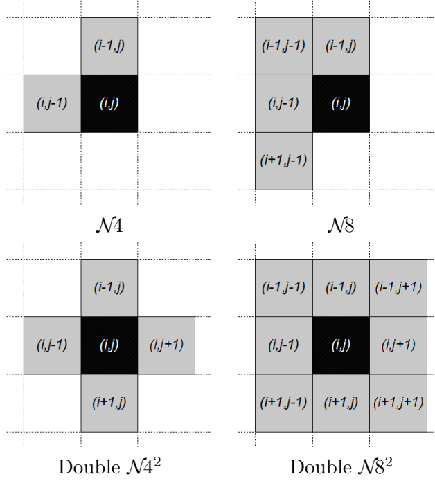
Figure 3: Neighborhoods \mathcal{N}4 and \mathcal{N}8 (right) of a pixel (i, j) are used to formulate \Phi(u) . The double neighborhoods \mathcal{N}4^2 and \mathcal{N}8^2 appear in the gradient of \Phi(u) , see (7).
