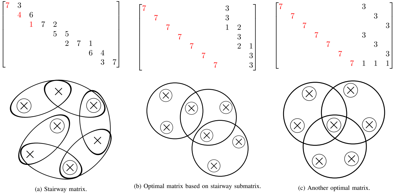
Fig. 2: Three communication matrices in the case 7 \times 10 and their representation as repartitioning hypergraph. Zero elements in matrices are not shown. The elements in red are those who remain in place during communications, others will migrate.
