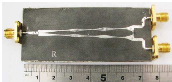
Figure 6 The photo of the fabricated power divider of [1, 2.8, 4.5] GHz. [Color figure can be viewed in the online issue, which is available at wileyonlinelibrary.com .]
