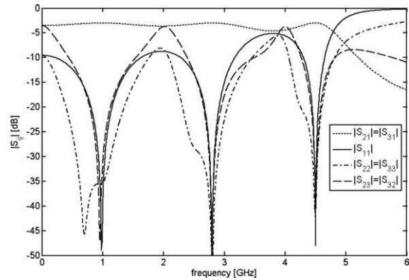
Figure 5 The amplitude of the scattering parameters of power divider of [1, 2.8, 4.5] GHz.
