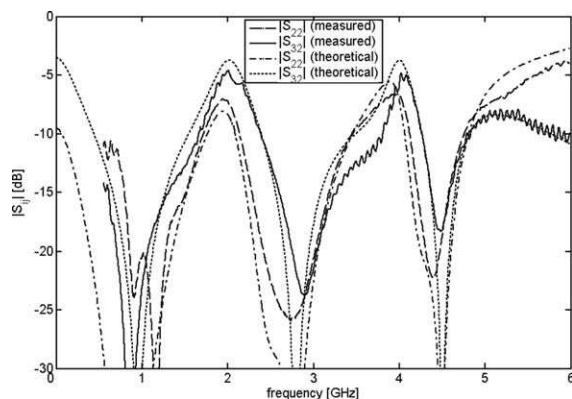
Figure 8 The measured and theoretical parameters |S_{22}| and |S_{32}| of the fabricated power divider.
