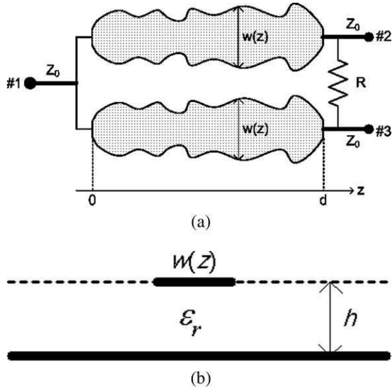
Figure 1 (a) Diplexer with two MNTLs (b) The cross section of an MNTL.
