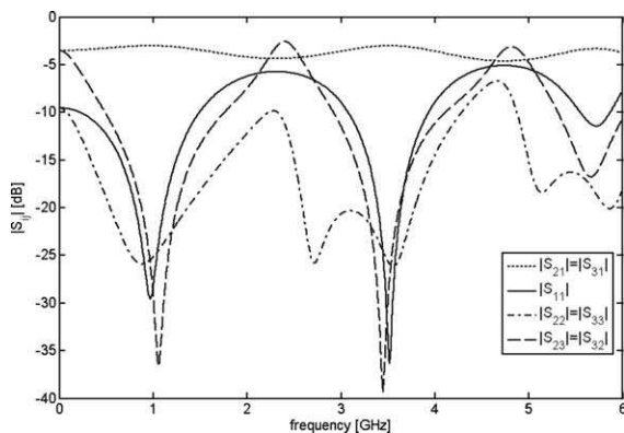
Figure 4 The amplitude of the scattering parameters of power divider of [1, 3.5] GHz.
