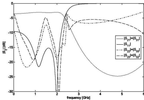
Figure 3 The amplitude of the scattering parameters of power divider of [1, 2] GHz.
