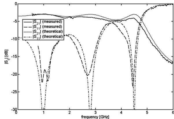
Figure 7 The measured and theoretical parameters |S_{11}| and |S_{21}| of the fabricated power divider.
