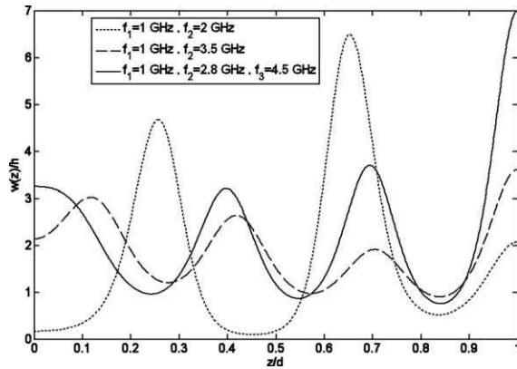
Figure 2 The normalized width function w(z)/h for three designed power dividers.
