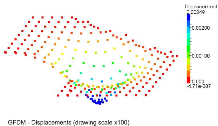
Figure 4: Deformed plate using GFDM
