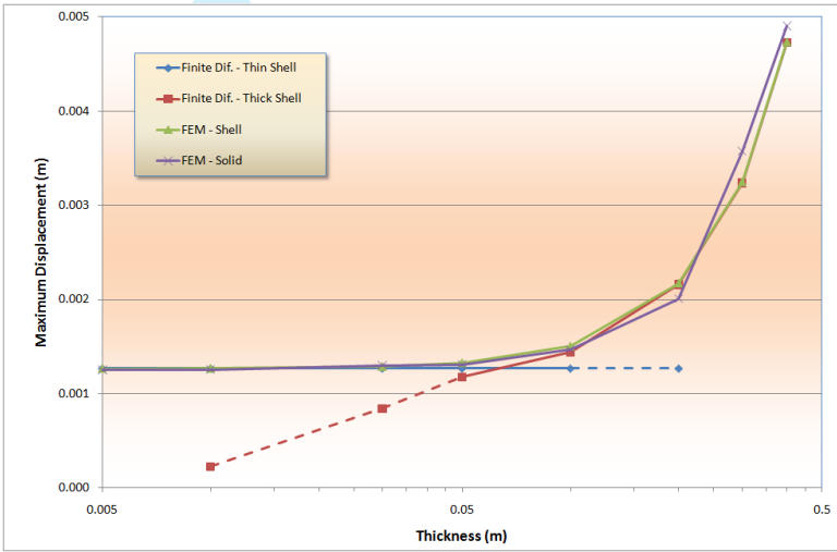
Figure 2: Comparison between different numerical methods at the node (0.5,0.5) for the fixed 1 × 1 plate as the plate thickness is increased
