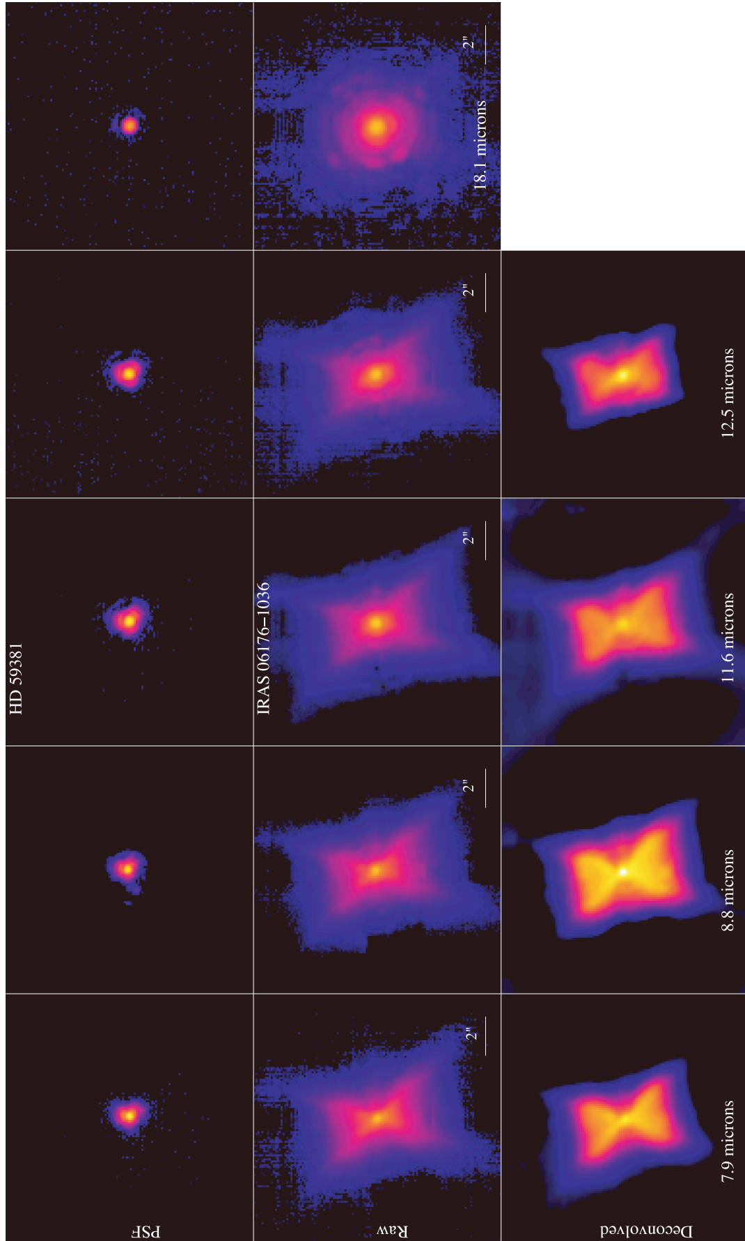
Figure B1. Michelson/Gemini-North images of IRAS 06176 (The Red Rectangle). North is up and east left.
