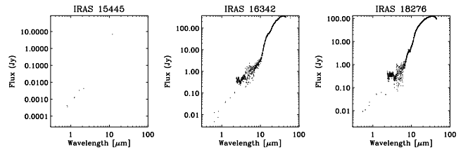
Figure 2. SED of the resolved objects with an equatorial dark lane.
