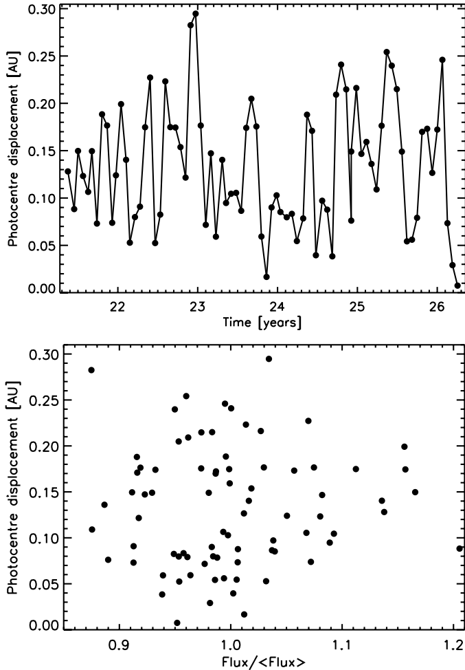
Fig. 5. Top panel: modulus of the photocentre displacement as a function of time. Bottom panel: photocentre displacement as a function of the integrated flux in the Gaia G band, \int_{3250 \text{ \AA}}^{10300 \text{ \AA}} F_{\lambda} d\lambda , normalised by the temporal average integrated flux.
