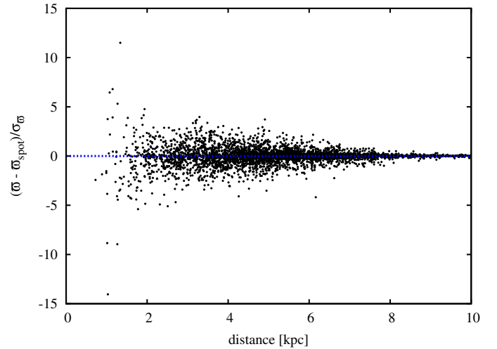
Fig. 21. Comparison of parallaxes for supergiant stars with and without surface brightness asymmetries (spots), normalised to \sigma_w . The stars falling on the horizontal line with ordinate 0 are very reddened stars, are consequently quite faint, and therefore have large errors on their astrometric measurements and thus on their parallax.
