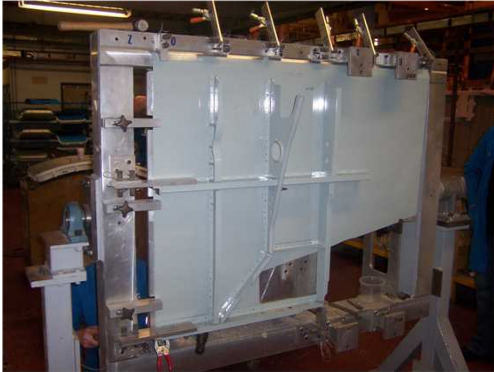
Uplock and Apron Assembly (With Fixture) 150x112mm (96 x 96 DPI)
