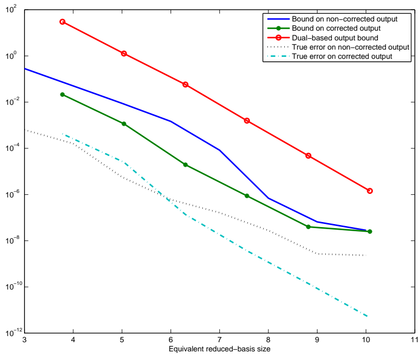
Figure 2: Comparison between the mean error bound (corr. and non-corr. outputs), the mean dual-based error bound, and the true (corr. and non-corr.) errors, for different reduced basis sizes.
