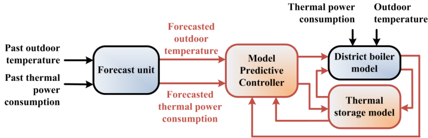
Figure 1. The OptiEnR project. In red, the proposed controlled thermal storage tank.
