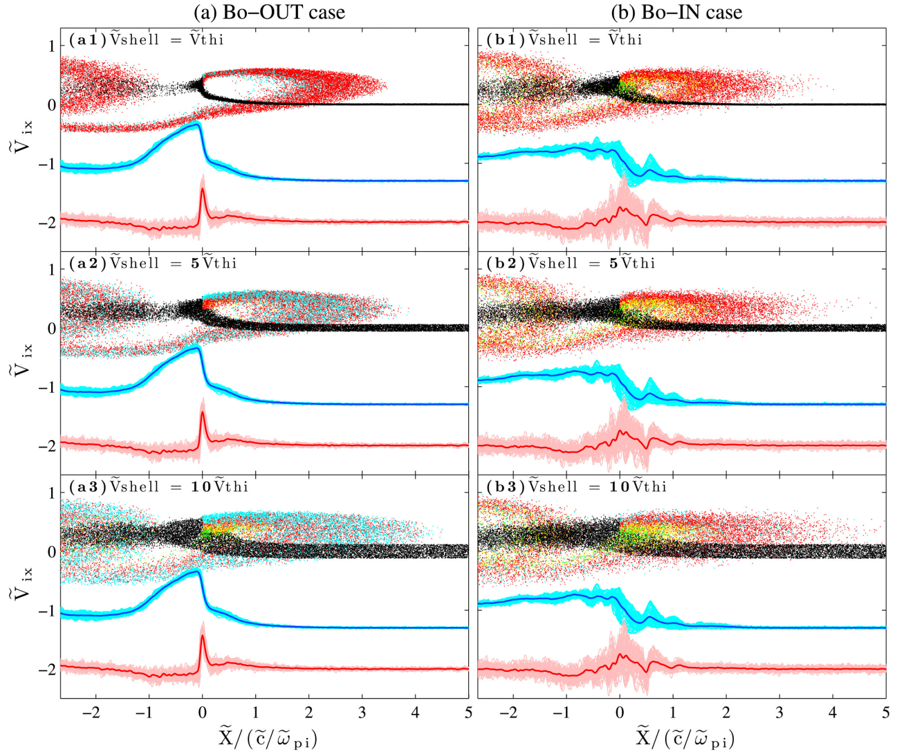
Figure 13. Ion phase space ( \tilde{V}_{ix}-\tilde{X} ) of ions issued from 2-D test particles simulations for three different initial shell velocities \tilde{V}_{shell} = 1, 5 and 10\tilde{V}_{thi} for the non-averaged shock profiles (i.e., front rippling included). Results are shown respectively for (a) “ B_0 -OUT” and (b) “ B_0 -IN” configurations. Spatial coordinate is normalized versus the ion inertial length \tilde{c}/\tilde{\omega}_{pi} . The ramp location is used as the origin \tilde{x} = 0 of the plot. Colors code is as follows: incoming and DT ions (black), SDA-C ions (cyan), SDA-NC ions (red), SSA-O ions (yellow) and SSA-M ions (green). For reference, the non-averaged fields of the shock profile \tilde{B}_z (cyan) and \tilde{E}_x (magenta) (as in Figure 12) are shown in each panel. The corresponding y-averaged fields \tilde{B}_z (blue) and \tilde{E}_x (red) are also shown for reference as in Figure 3.
