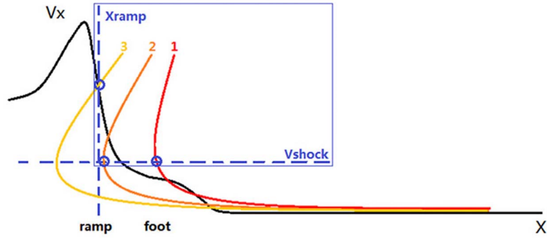
Figure 2. Sketch of typical reflected ion trajectories. The red, orange and yellow curves illustrate respectively trajectories of an SSA/SDA ion reflected within the foot, at the ramp and of an SDA ion reflected after the overshoot (herein so-called SDA-C ion); the blue circles indicate the location where the incident ion is defined as reflected, and is classified into SSA and SDA groups by using the criteria described in the text.
