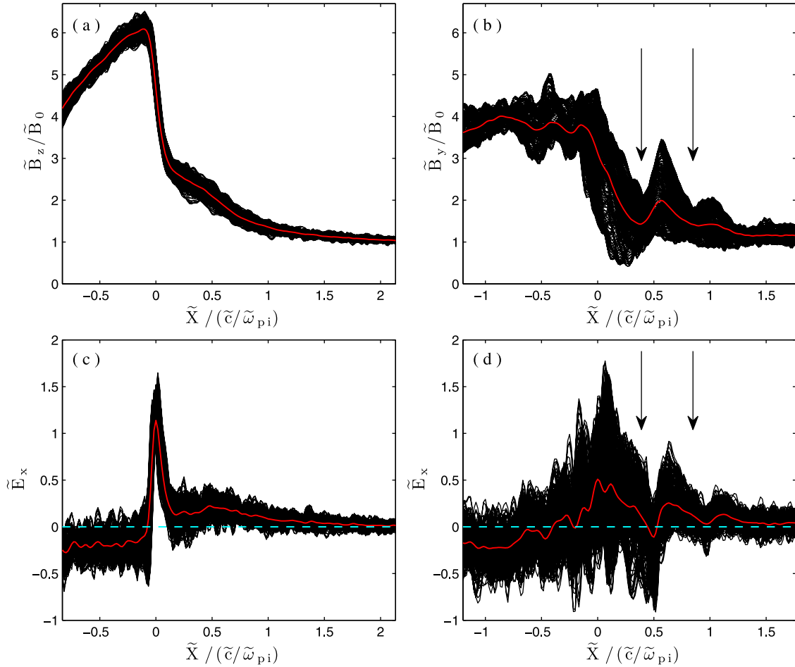
Figure 12. Profiles of the main magnetic field and of the electrostatic field \tilde{E}_x for the (a and c) “ B_0 -OUT” and (b and d) “ B_0 -IN” configurations. In each panel, the different x-profiles measured for all y-values are superimposed; the corresponding y-averaged profile (red) is indicated too. The ramp location is used as the origin \tilde{x} = 0 of the plot.
