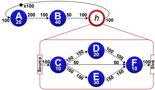
Fig. 2. Interface Based SDF (IBSDF) graph
