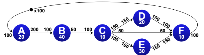
Fig. 4. Flattened Synchronous Data-Flow
