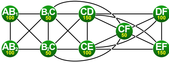
Fig. 6. Memory Exclusion Graph
