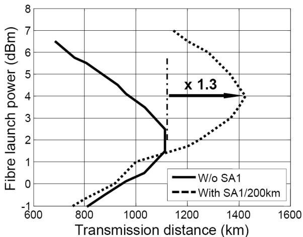
Fig. 32. A map of BER=10^{-4} versus launch power and transmission distance w/o and with regeneration every 200 km.
