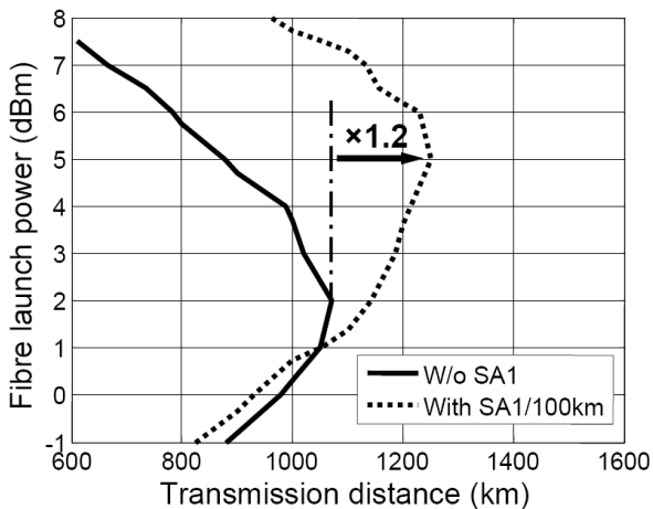
Fig. 31. A map of BER=10^{-4} versus launched power and transmission distance with and without regeneration every 100 km.
