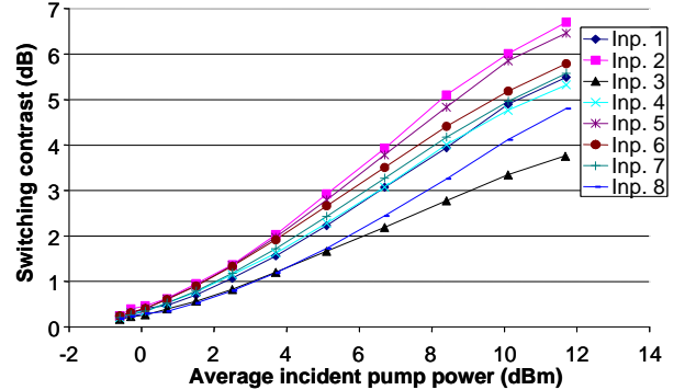
Fig. 5. Experimental switching contrast of SA module versus average incident pump power
