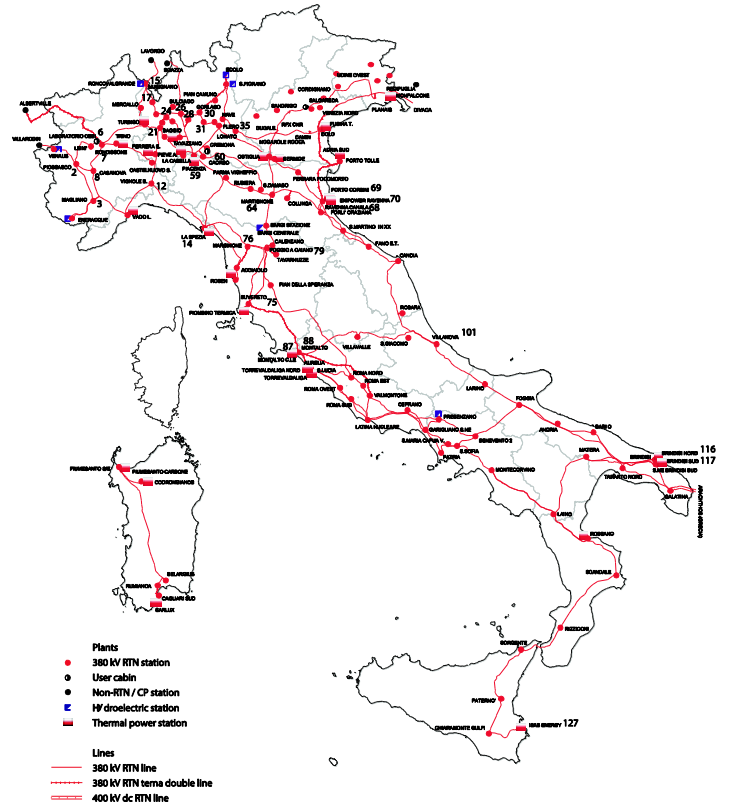
Figure 1. The 380 kV Italian power transmission network (TERN 2002, Rosato, Bologna et al. 2007).
