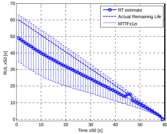
Figure 10 RT estimation for a trajectory which does not exceed any safety threshold value, although a failure sequence has occurred
