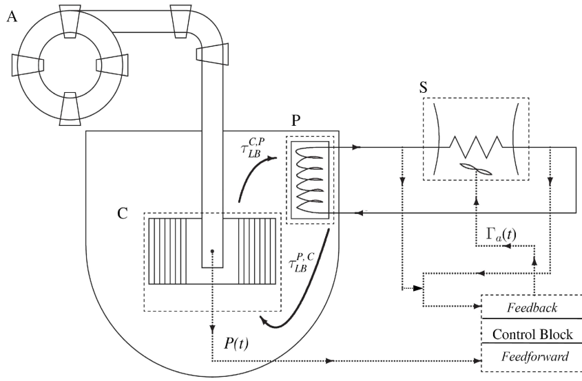
Figure 5 LBE-XADS simplified schematics. A = Accelerator; C = core; P = primary heat exchanger; S = secondary heat exchanger
