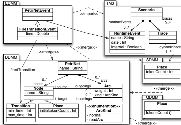
Fig. 6: PETRINET metamodels
