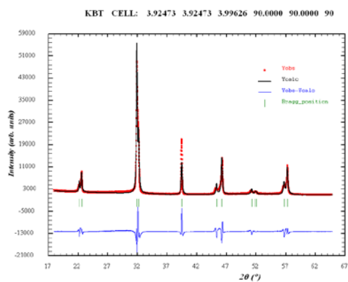
Figure 5 X-ray diffraction refinement diagram for the K_{1/2}Bi_{1/2}TiO_3 (KBT), compound.
