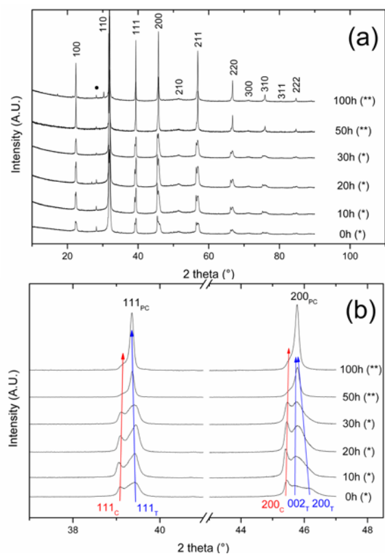
Figure 3 (a) X-ray diffraction diagrams of the K_{1/2}Bi_{1/2}Ti_{0.90}Zr_{0.10}O_3 composition for different annealing times. (★: samples annealed successively three times for 10h, ★★: same initial batch annealed directly two times for 50h).
