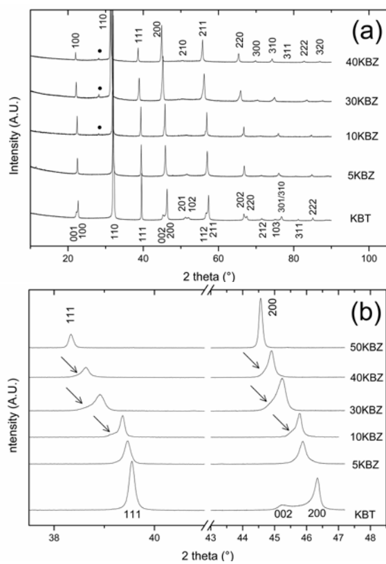
Figure 4 (a) X-ray diffraction diagrams of K_{1/2}Bi_{1/2}Ti_{(1-x)}Zr_xO_3 compounds (• = ZrO_2 ), (b) detail for the (111) and (200) peaks. The x = 0.05 and x = 0.1 were annealed at 1000^\circ\text{C} for 50h, x = 0.3 at 1000^\circ\text{C} for 10h, x = 0.4 and x = 0.5 are raw samples (The arrow shows the asymmetry indicating a departure from pure cubic symmetry).
