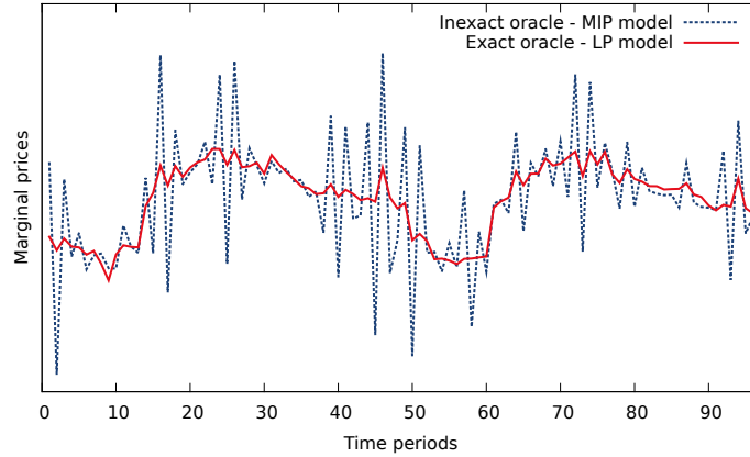
Fig. 1 Exact and inexact prices over time periods in EDF problem. For industrial privacy, price scales are not provided.
