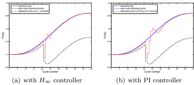
Fig. 10. Closed loop simulation with Hammerstein model.
