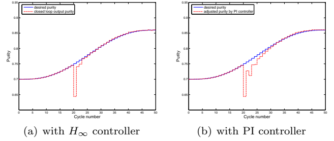
Fig. 11. Closed loop simulation with P.S.A model.
