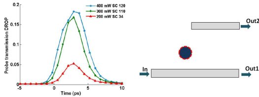
Fig. 1. Schematic representation of the AOG (right). Pump-probe operations in a three-ports AOG optimized design (left). The curves show the probe efficiency at the drop port for different control power injected into the structure. The corresponding values of the switching contrast (SC) are also indicated.
