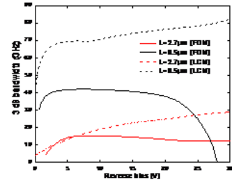
Fig. 3. Frequency response of the photodetector. LCM: constant low-field mobility model (dashed lines), FDM: field-dependent mobility model (solid lines).
