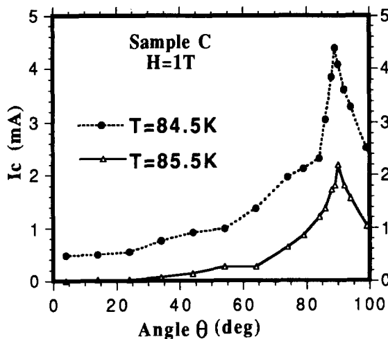
Figure 4. Angular dependence of I_c close to T_c for sample C.
