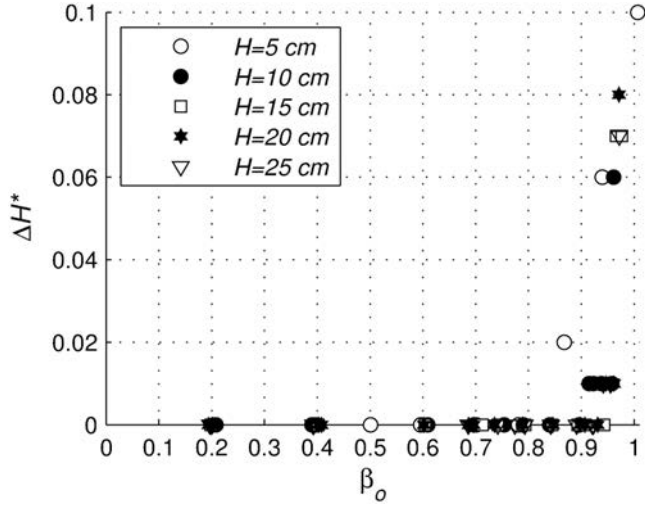
Figure 2. Bed expansion as a function of the initial fluidization rate, \beta_o , for different initial bed heights ( H ). \Delta H^* = (H_e - H)/H , where H is the initial (non-expanded) height and H_e is the expanded bed height. Bed expansion occurs when \beta_o > \beta_{oc} , (with \beta_{oc} \sim 0.8 for H = 5 cm and \beta_{oc} \sim 0.9 for H \geq 10 cm).
