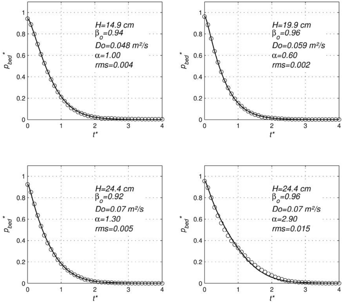
Figure 8. Experimental data (circles) and numerical fit (line) at the base of the tank for initially expanded mixtures ( \beta_o > \beta_{oc} ) using equations (15) and (16). In the figures, rms stands for root mean square error of the fitted curve respect to the experimental data.
