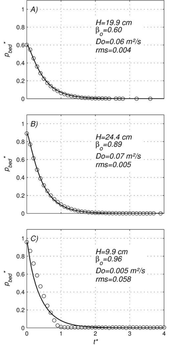
Figure 3. Experimental data (circles) and theoretical model (line) for the time variation of pore pressure at the base of the granular column for (a) \beta_o < \beta_{oc} , (b) \beta_o values lower but close to \beta_{oc} and (c) \beta_o > \beta_{oc} . For column height of the order of or greater than \sim 10 cm, \beta_{oc} \sim 0.9 . The solid line corresponds to the best fit curve with experimental data, adjusting the pore pressure diffusion coefficient, Do . In the figures, rms stands for root mean square error of the fitted curve respect to the experimental data.
