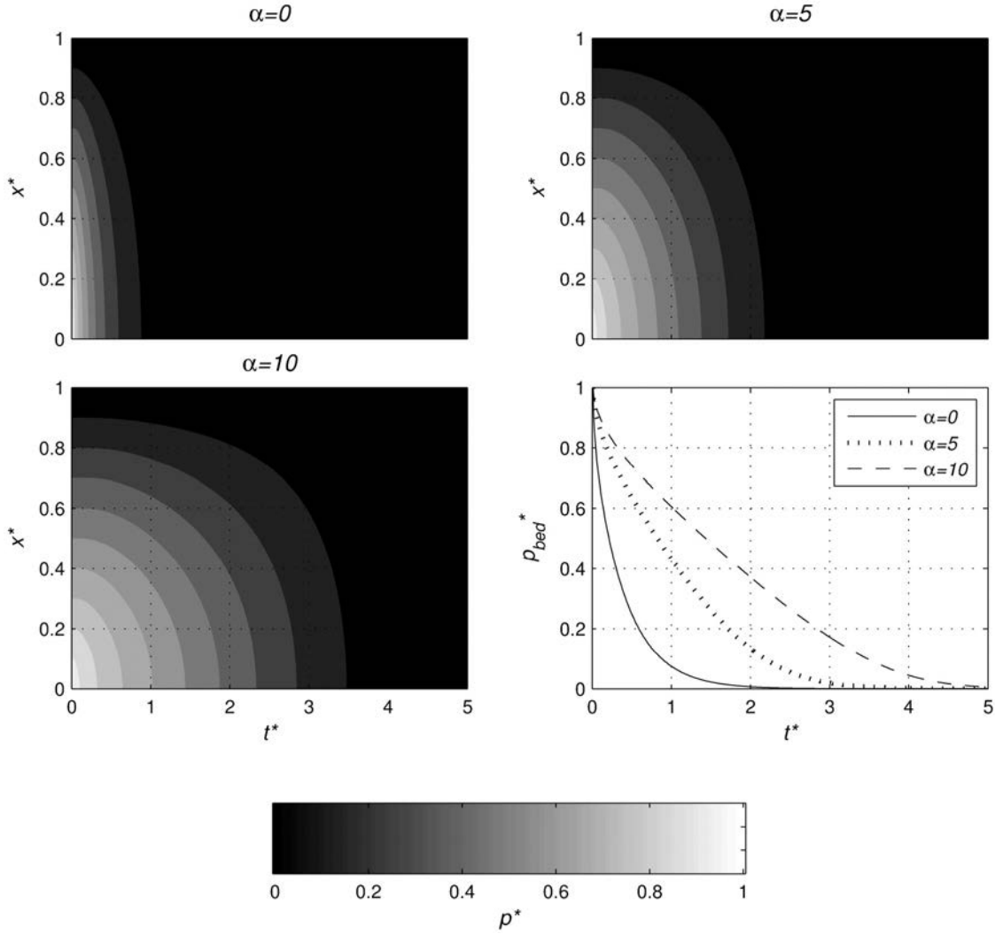
Figure 9. Vertical profile of the dimensionless pore pressure time evolution ( p^* ) for an initially fully fluidized granular bed and different \alpha values using equations (15) and (16). Values of \alpha vary in the range of 0 to 10 (Figure 7). The solutions shown for \alpha = 0 correspond to those of linear diffusion. The term p_{bed}^* at the right bottom corner represents the dimensionless pore fluid pressure at the base of the granular column. The color bar represents values of p^* .
