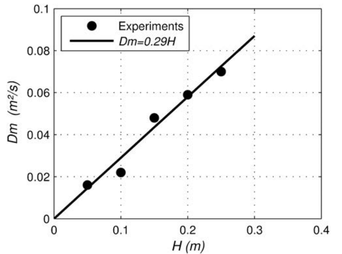
Figure 5. Linear dependence of Dm , the mean linear diffusion coefficient in the range 0.7 < \beta_o < \beta_{oc} ( \beta_{oc} \sim 0.8 for H = 5 cm and \beta_{oc} \sim 0.9 for H > 5 cm) in terms of the initial column height, H .
