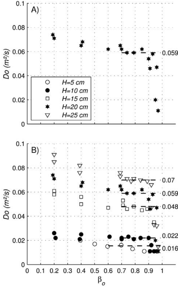
Figure 4. Variation of the pore pressure diffusion coefficient, Do , as a function of the initial degree of fluidization, \beta_o , obtained by fitting the experimental measurements at the base of the tank with the linear diffusion model ( D^* = 1 ). (a) Decrease of Do with \beta_o , tending to an almost constant value of Do in the range 0.7 < \beta_o < \beta_{oc} ( \beta_{oc} \sim 0.9 ). When \beta_o > 0.9 , an abrupt drop in Do is observed. (b) The same results but for different column heights ( \beta_{oc} \sim 0.8 for H = 5 cm and \beta_{oc} \sim 0.9 for H > 5 cm). Numbers on the right indicate values of Dm .
