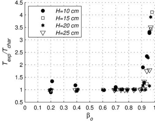
Figure 6. Ratio of characteristic diffusion time scales, T_{\text{exp}}/T_{\text{char}} , where T_{\text{exp}} represents a characteristic dimensionless diffusion time scale estimated by means of the measured basal pore fluid pressure evolution and T_{\text{char}} corresponds to a characteristic dimensionless diffusion time scale based in the linear solution for the pore fluid pressure equation. The experimental pore pressure diffusion time scale becomes larger than the theoretical linear diffusion time scale at \beta_o > \beta_{oc} . Values greater than 1 for \beta_o \sim 0.2 and \beta_o \sim 0.4 and H = 10 cm are attributed to errors in the experimental procedure.
