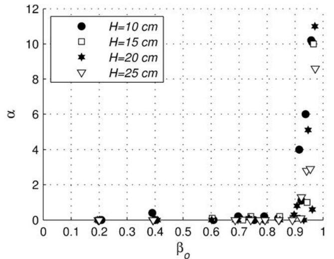
Figure 7. Fitted values of \alpha as a function of \beta_o for different initial heights. For \beta_o < \beta_{oc} , when the bed is not expanded and the linear diffusion model is applicable, values of \alpha are equal to zero.
