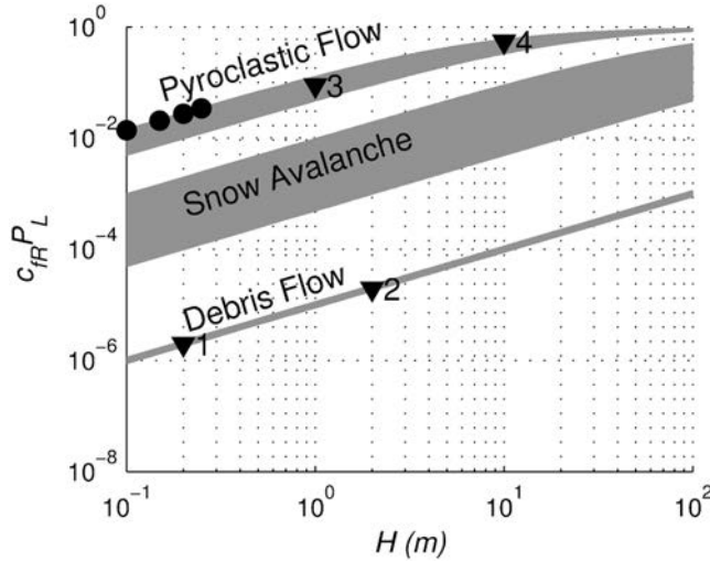
Figure 11. Estimates of c_{fr} P_L for different types of geophysical granular flows and our laboratory experiments. Reference values of the pore fluid compressibility ( c_{fr} ) are assumed to be 5 \times 10^{-10} \text{ Pa}^{-1} and 10^{-5} \text{ Pa}^{-1} in the case of water-particle (debris flow) and air-particle (pyroclastic flows and snow avalanches) mixtures, respectively. Mixture densities are assumed within the range 1800\text{--}2300 \text{ kg/m}^3 for debris flows [Iverson, 1997; Iverson and Vallance, 2001; Hauser, 2002], 10\text{--}1000 \text{ kg/m}^3 for snow avalanches [McClung and Schaerer, 1993; Turnbull and McElwaine, 2007], and 500\text{--}1500 \text{ kg/m}^3 for pyroclastic flows [Druitt, 1998; Freundt et al., 2000]. Flow heights, H , are in the range 0.1\text{--}100 \text{ m} . Black dots represent the values of c_{fr} P_L in the present experiments, while black triangles correspond to estimations of c_{fr} P_L values computed out of the granular flow data reported by Iverson and Denlinger [2001]: 1) experimental USGS debris flows, 2) Yake Lake, debris flow, 3) small-volume pumice pyroclastic flow deposits of Mount St. Helens and 4) Elm rock Avalanche.
