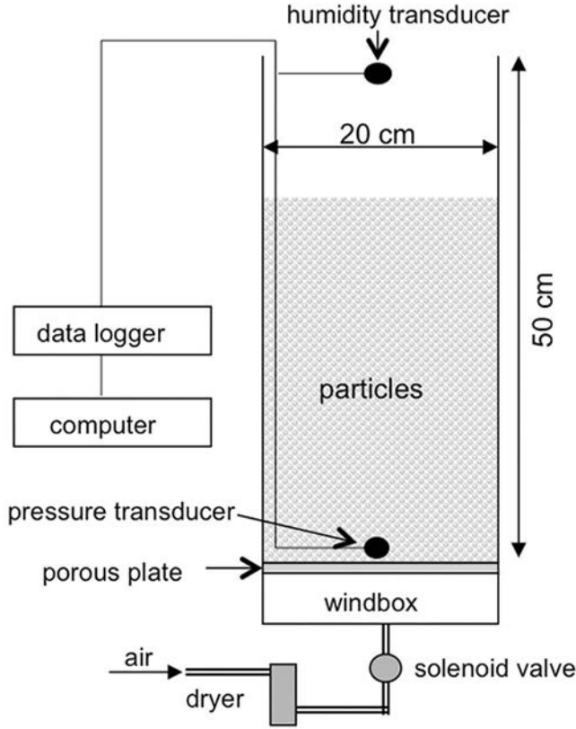
Figure 1. Sketch of the experimental device.
