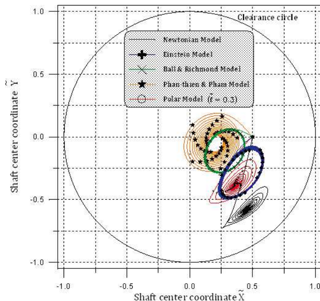
Fig. 17. Shaft trajectories for 30% particle concentration.
