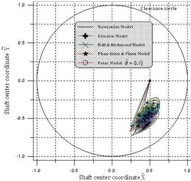
Fig. 11. Shaft trajectories for 10% concentration of particles.
