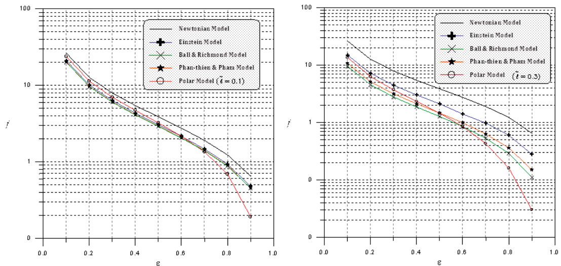
Fig. 7. Friction factor versus static eccentricity ratio for different rheological models ( \Phi = 10\% left and \Phi = 30\% right).
