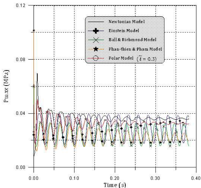
Fig. 16. Maximum pressure evolution with time for 30% particle concentration.
