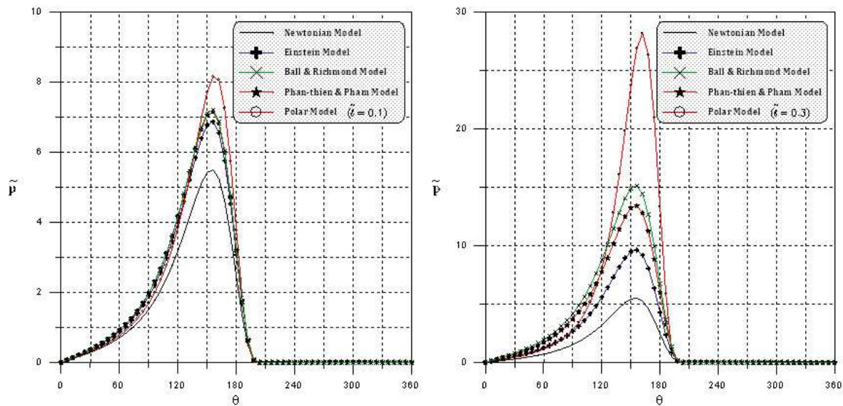
Fig. 4. Dimensionless pressure distribution for different rheological models ( \Phi = 10\% left, and \Phi = 30\% right; \varepsilon = 0.7 ).
