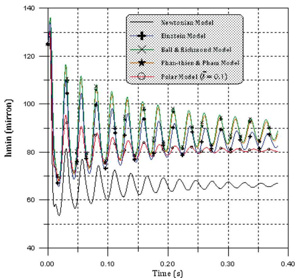
Fig. 9. Minimum film thickness evolution with time for 10% particle concentration.
