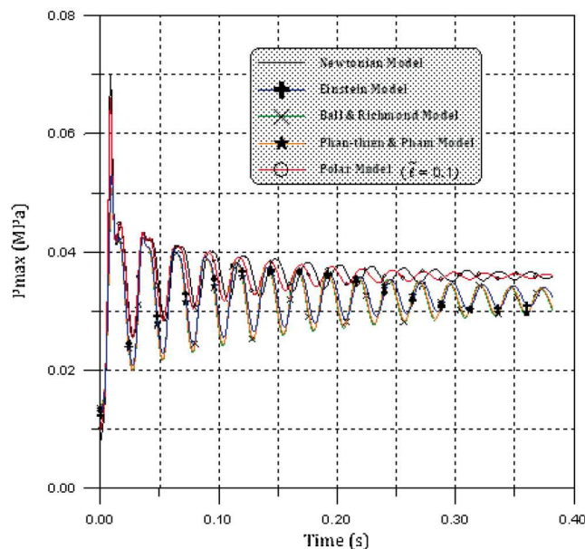
Fig. 10. Maximum pressure evolution with time for 10% particle concentration.
