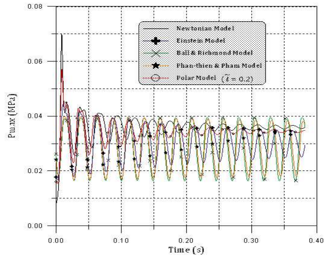
Fig. 13. Maximum pressure evolution with time for 20% particle concentration.
