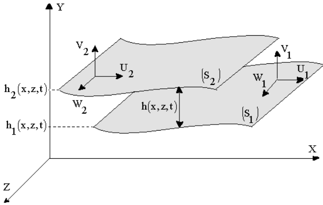
Fig. 2. Geometry and kinematics of contact.
