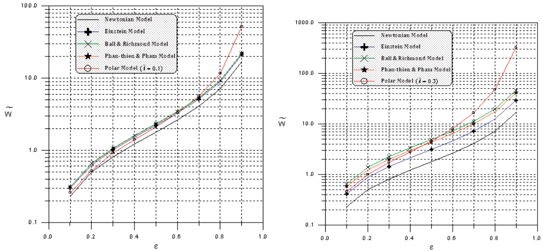
Fig. 5. Dimensionless carrying capacity versus eccentricity ratio for different rheological models ( \Phi = 10\% left, and \Phi = 30\% right).
