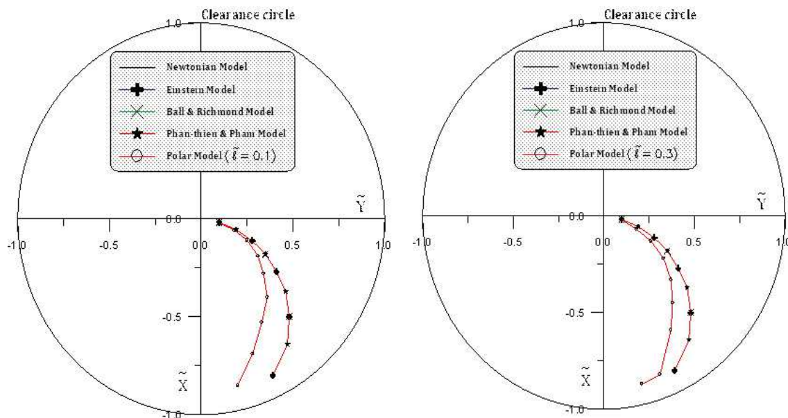
Fig. 8. Static attitude angle versus static eccentricity ratio for different rheological models ( \Phi = 10\% left and \Phi = 30\% right).
