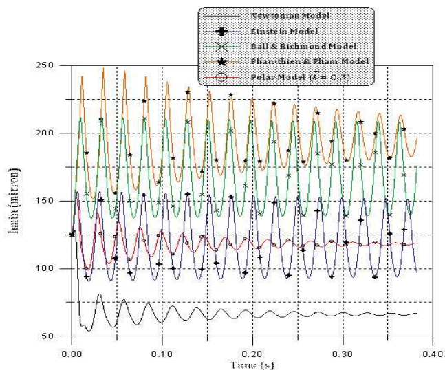
Fig. 15. Minimum film thickness evolution with time for 30% particle concentration.
