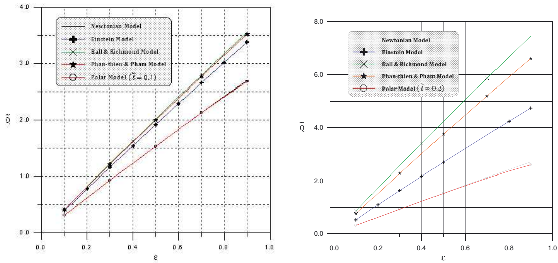
Fig. 6. Dimensionless side leakage flow versus static eccentricity ratio for different rheological models ( \Phi = 10\% left, and \Phi = 30\% right).
