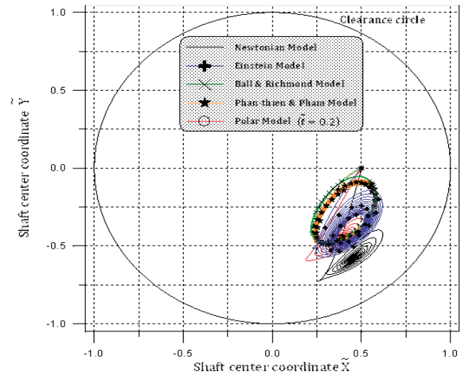
Fig. 14. Shaft trajectories for 20% particle concentration.
