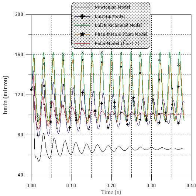
Fig. 12. Minimum film thickness evolution with time for 20% particle concentration.
