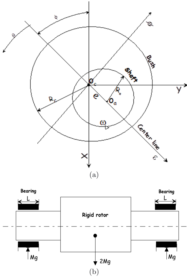
Fig. 3. Rotor-bearing system and system axes. (a) Cross-section of the bearing. (b) Schematic of the system.
