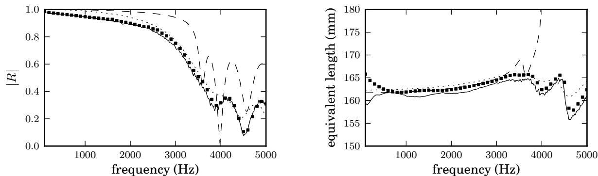
Figure 5: Magnitude of the reflectance (left) and equivalent length (right) of a pipe with 10 toneholes: experimental results (solid), FEM simulation results (squares), calculations with external interactions (TMMI, dotted) and calculations without interactions (TMM, dashed).
